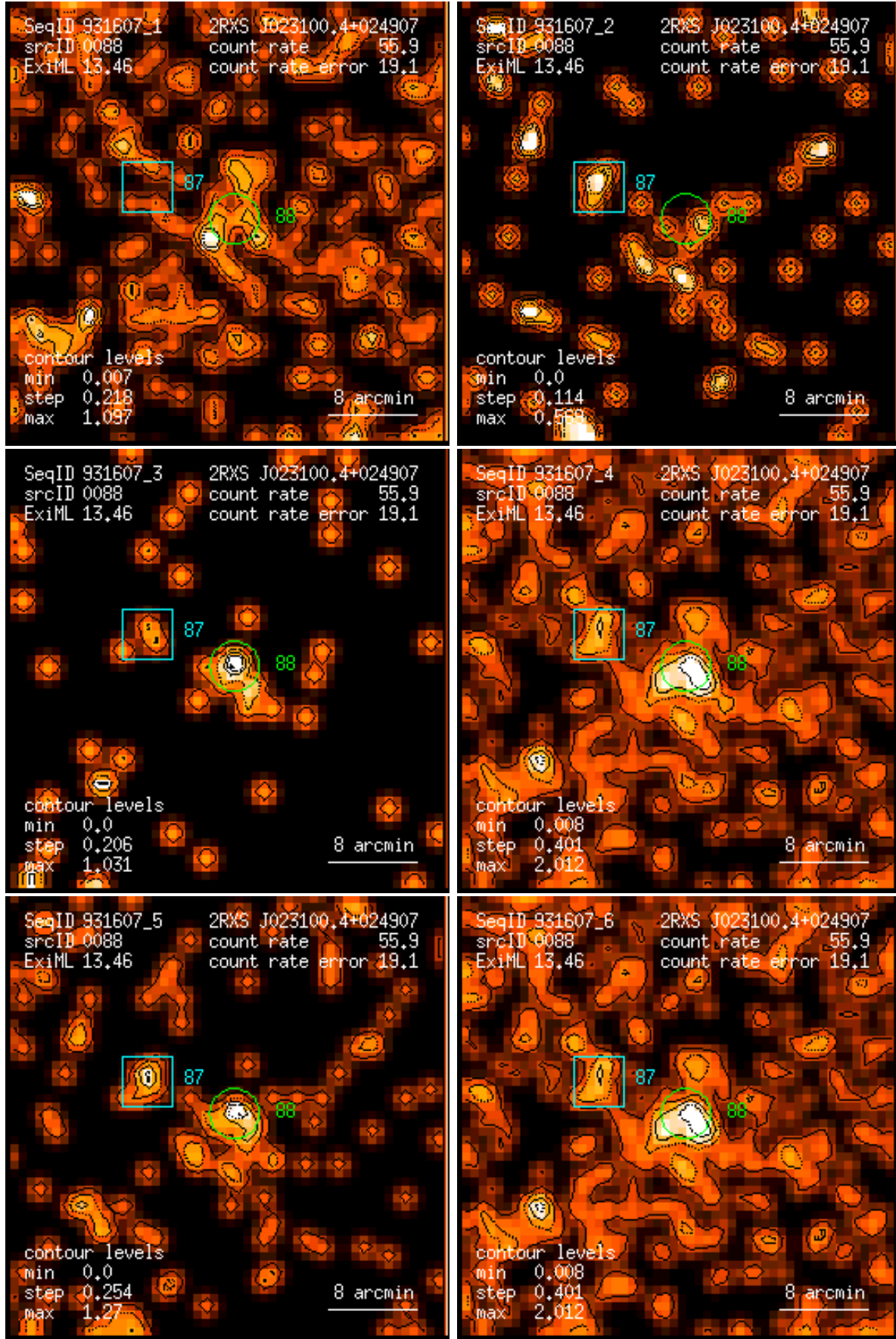
Figure 88: RASS 931607: detection 0088: band rate images, Gaussian filter: (1) PSPC channels 11 – 41, (2) 52 – 90, (3) 91 – 201, (4) 11 – 235, (5) 52 – 201, (6) 11 – 201. Broad band rates in counts/ks. Band rate contour levels in counts/ks/arcmin 2 .
