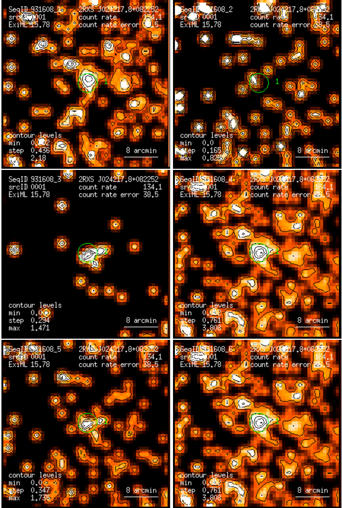
Figure 1: RASS 931608: detection 0001: band rate images, Gaussian filter: (1) PSPC channels 11 – 41, (2) 52 – 90, (3) 91 – 201, (4) 11 – 235, (5) 52 – 201, (6) 11 – 201. Broad band rates in counts/ks. Band rate contour levels in counts/ks/arcmin 2 .
