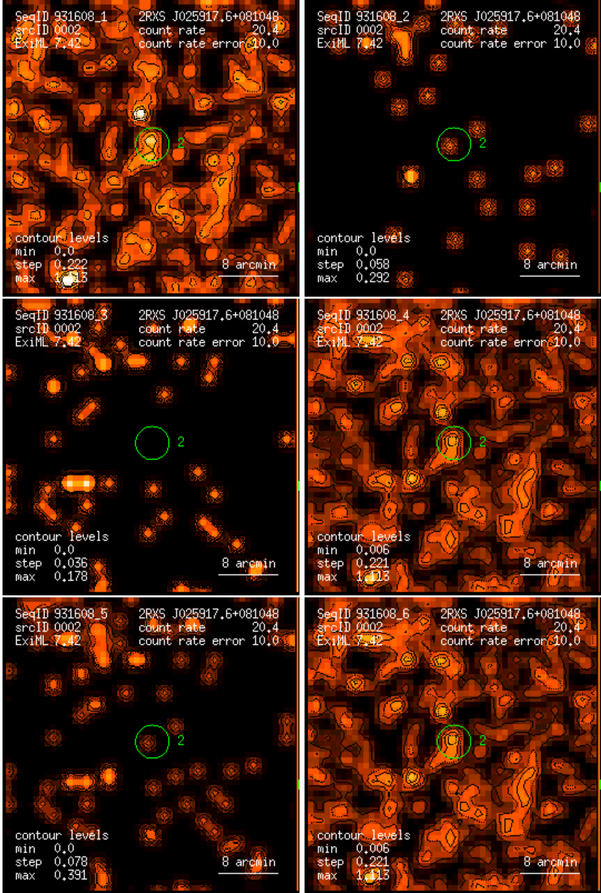
Figure 2: RASS 931608: detection 0002: band rate images, Gaussian filter: (1) PSPC channels 11 – 41, (2) 52 – 90, (3) 91 – 201, (4) 11 – 235, (5) 52 – 201, (6) 11 – 201. Broad band rates in counts/ks. Band rate contour levels in counts/ks/arcmin 2 .
