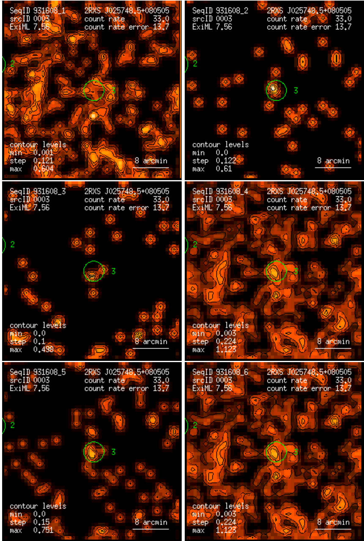
Figure 3: RASS 931608: detection 0003: band rate images, Gaussian filter: (1) PSPC channels 11 – 41, (2) 52 – 90, (3) 91 – 201, (4) 11 – 235, (5) 52 – 201, (6) 11 – 201. Broad band rates in counts/ks. Band rate contour levels in counts/ks/arcmin 2 .
