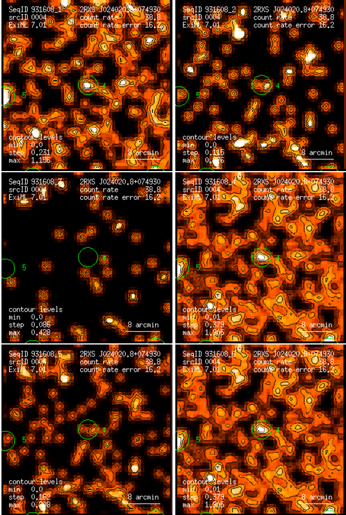
Figure 4: RASS 931608: detection 0004: band rate images, Gaussian filter: (1) PSPC channels 11 – 41, (2) 52 – 90, (3) 91 – 201, (4) 11 – 235, (5) 52 – 201, (6) 11 – 201. Broad band rates in counts/ks. Band rate contour levels in counts/ks/arcmin 2 .
