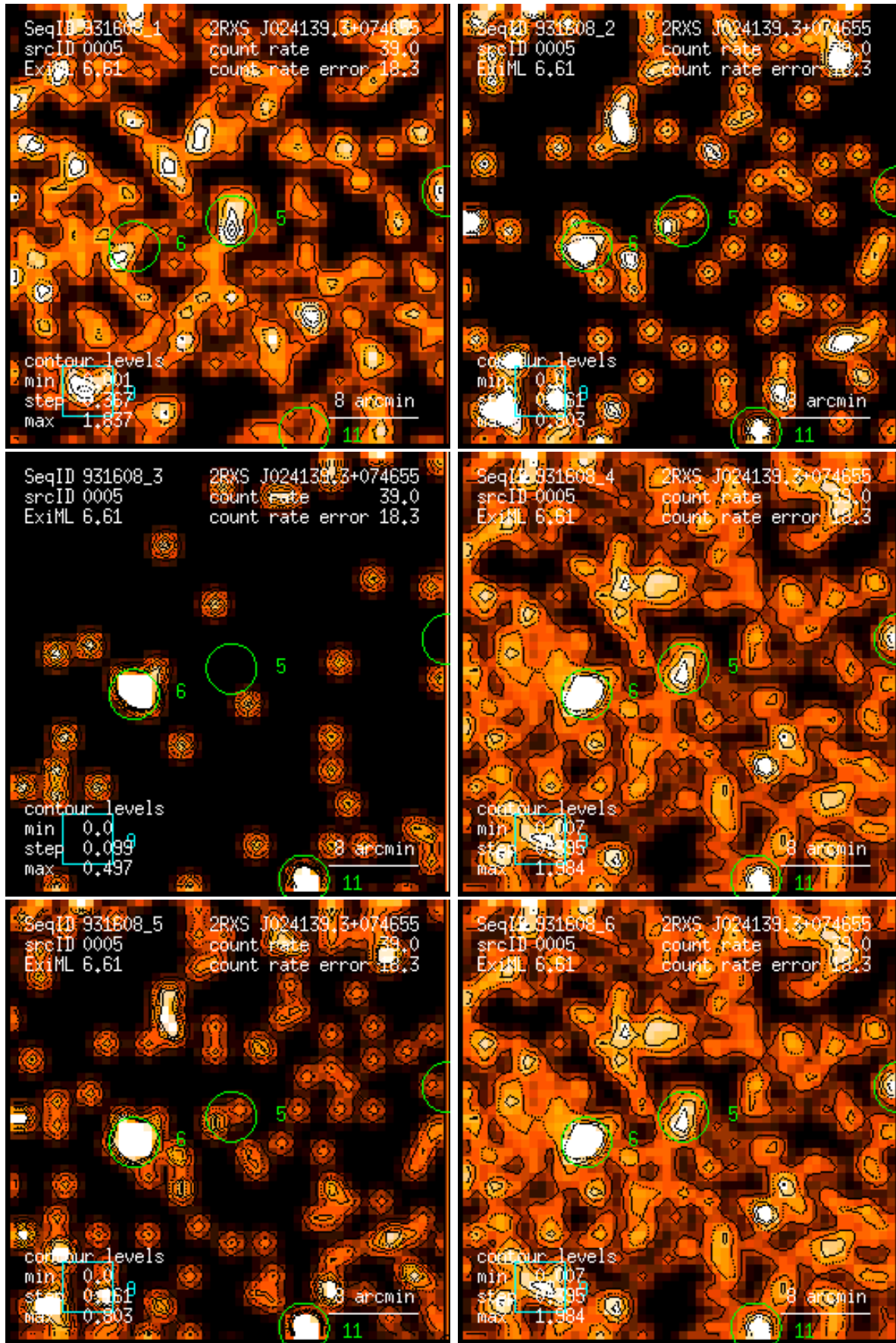
Figure 5: RASS 931608: detection 0005: band rate images, Gaussian filter: (1) PSPC channels 11 – 41, (2) 52 – 90, (3) 91 – 201, (4) 11 – 235, (5) 52 – 201, (6) 11 – 201. Broad band rates in counts/ks. Band rate contour levels in counts/ks/arcmin 2 .
