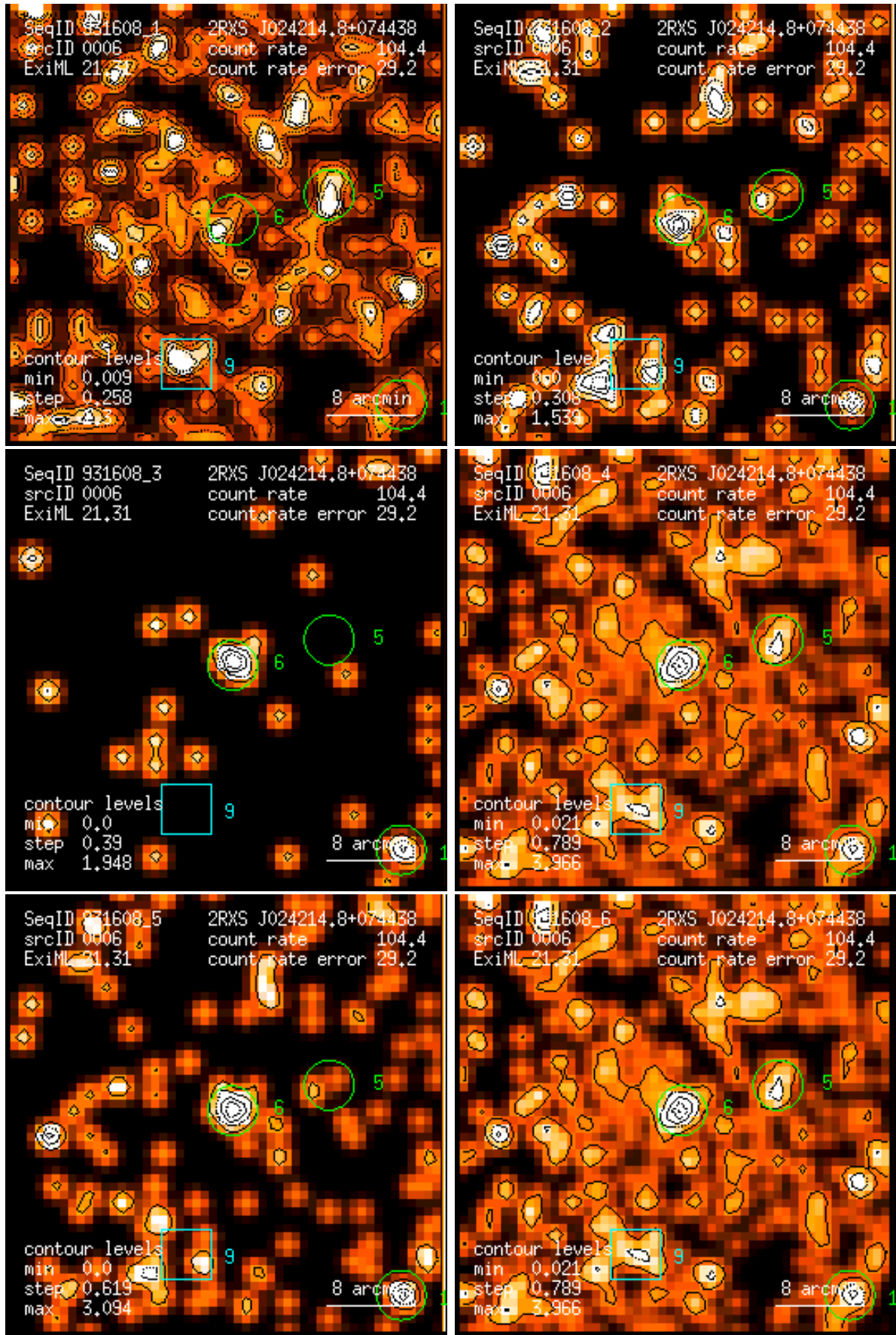
Figure 6: RASS 931608: detection 0006: band rate images, Gaussian filter: (1) PSPC channels 11 – 41, (2) 52 – 90, (3) 91 – 201, (4) 11 – 235, (5) 52 – 201, (6) 11 – 201. Broad band rates in counts/ks. Band rate contour levels in counts/ks/arcmin 2 .
