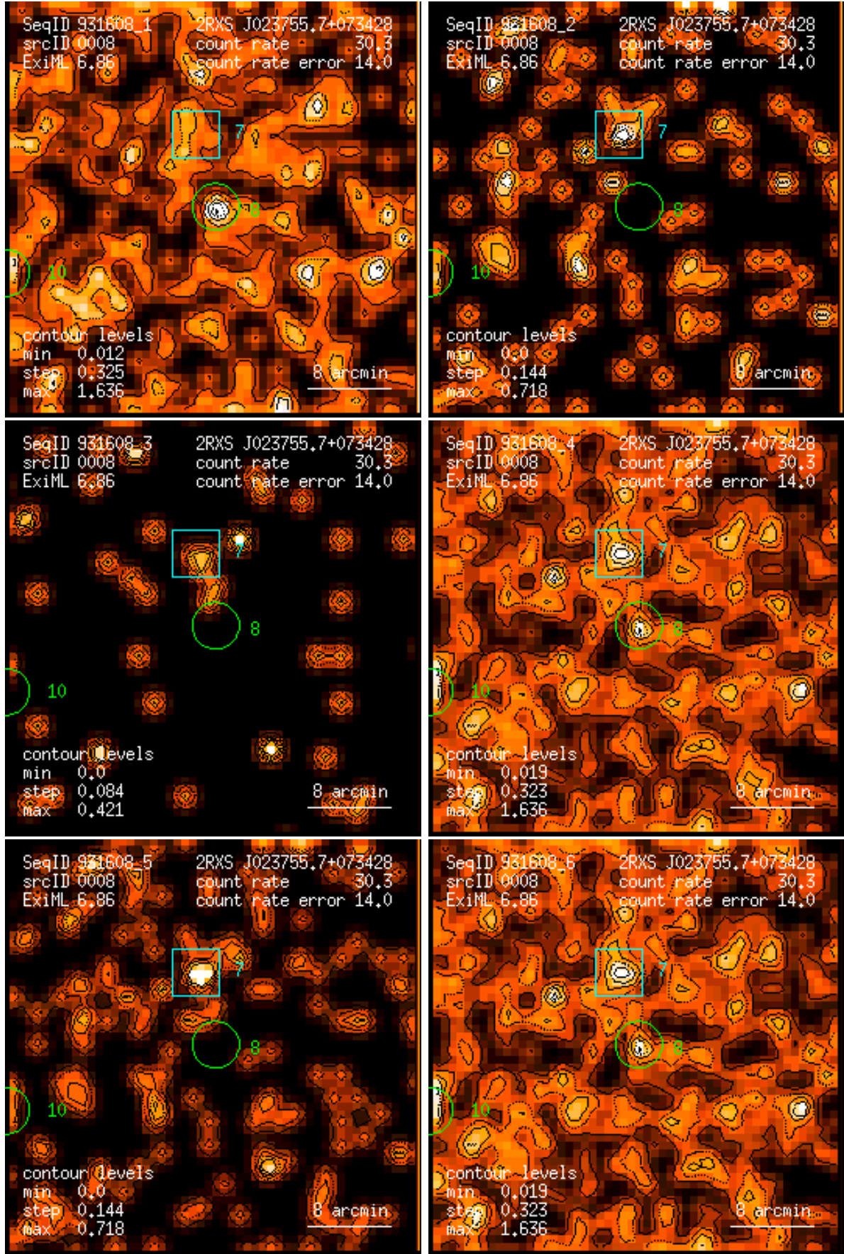
Figure 8: RASS 931608: detection 0008: band rate images, Gaussian filter: (1) PSPC channels 11 – 41, (2) 52 – 90, (3) 91 – 201, (4) 11 – 235, (5) 52 – 201, (6) 11 – 201. Broad band rates in counts/ks. Band rate contour levels in counts/ks/arcmin 2 .
