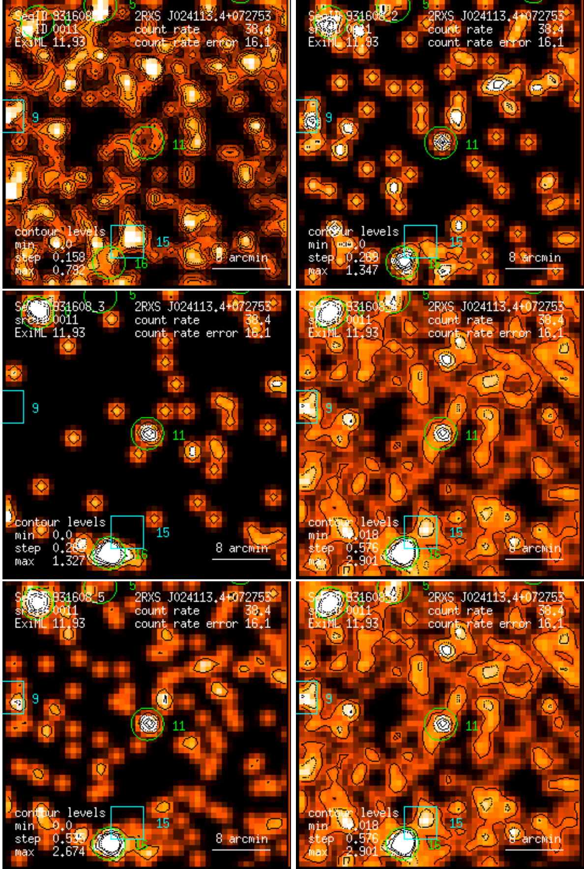
Figure 11: RASS 931608: detection 0011: band rate images, Gaussian filter: (1) PSPC channels 11 – 41, (2) 52 – 90, (3) 91 – 201, (4) 11 – 235, (5) 52 – 201, (6) 11 – 201. Broad band rates in counts/ks. Band rate contour levels in counts/ks/arcmin 2 .
