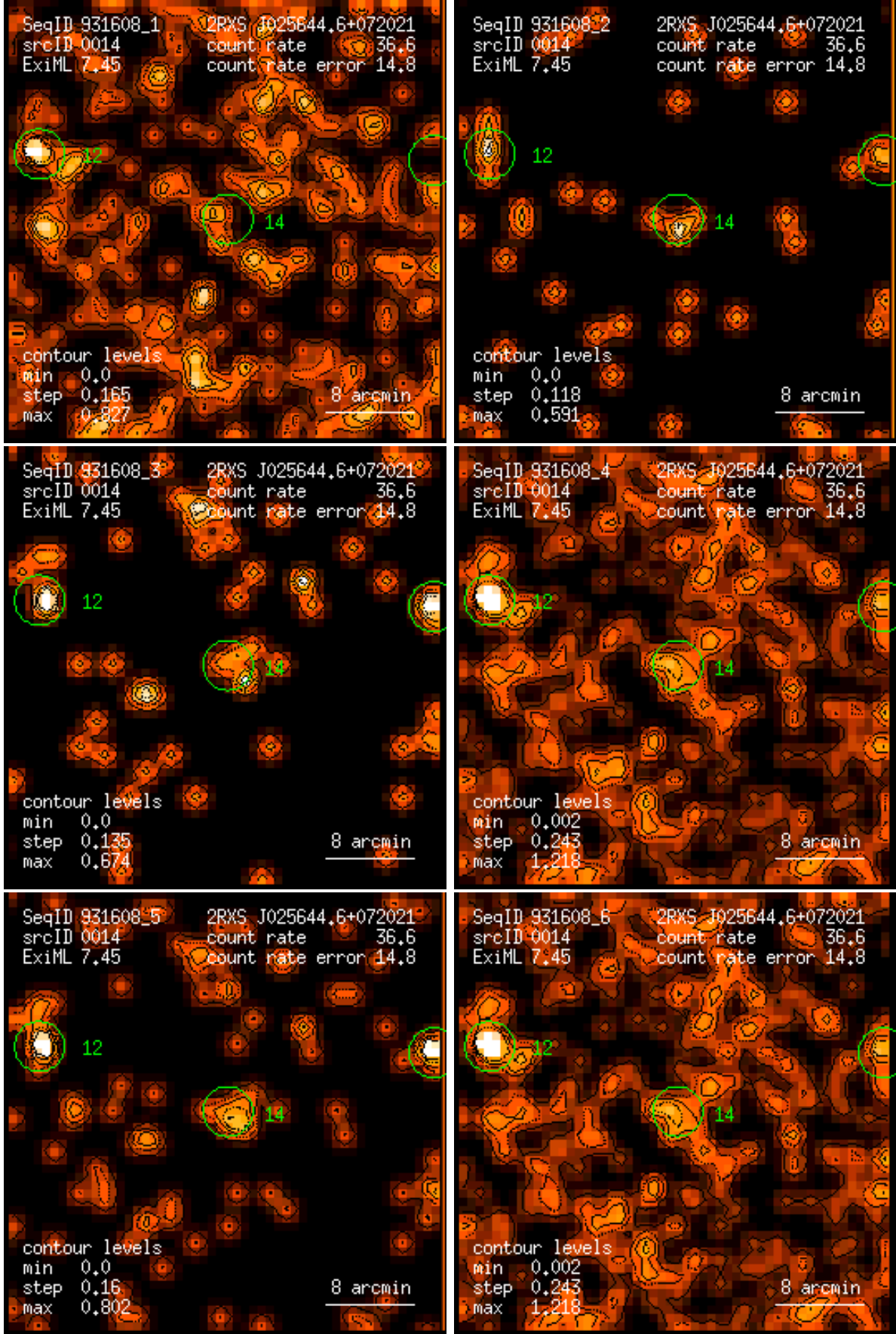
Figure 14: RASS 931608: detection 0014: band rate images, Gaussian filter: (1) PSPC channels 11 – 41, (2) 52 – 90, (3) 91 – 201, (4) 11 – 235, (5) 52 – 201, (6) 11 – 201. Broad band rates in counts/ks. Band rate contour levels in counts/ks/arcmin 2 .
