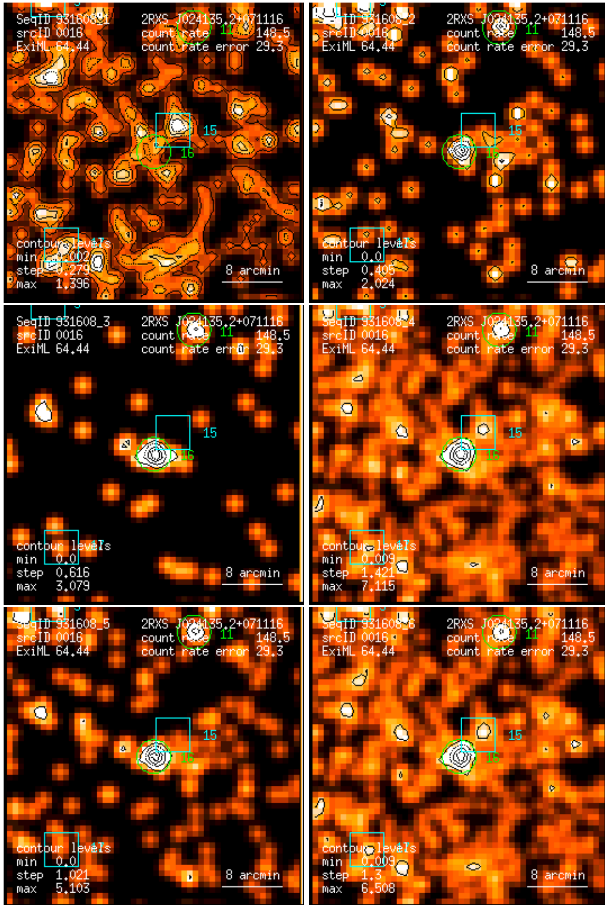
Figure 16: RASS 931608: detection 0016: band rate images, Gaussian filter: (1) PSPC channels 11 – 41, (2) 52 – 90, (3) 91 – 201, (4) 11 – 235, (5) 52 – 201, (6) 11 – 201. Broad band rates in counts/ks. Band rate contour levels in counts/ks/arcmin 2 .
