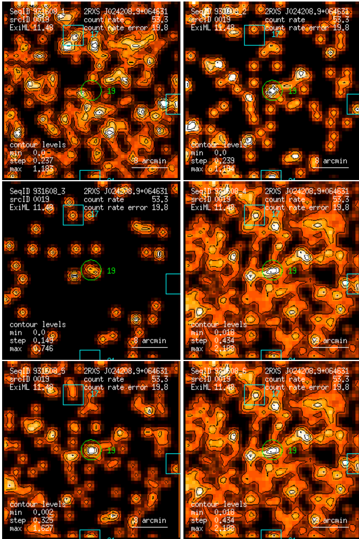
Figure 19: RASS 931608: detection 0019: band rate images, Gaussian filter: (1) PSPC channels 11 – 41, (2) 52 – 90, (3) 91 – 201, (4) 11 – 235, (5) 52 – 201, (6) 11 – 201. Broad band rates in counts/ks. Band rate contour levels in counts/ks/arcmin 2 .
