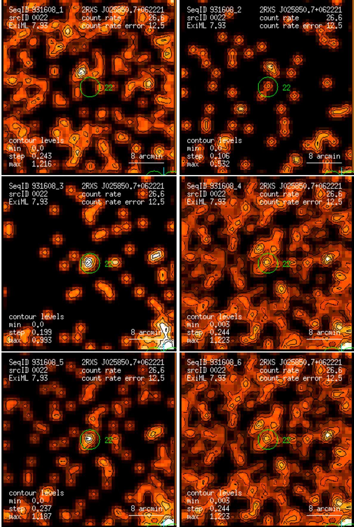
Figure 22: RASS 931608: detection 0022: band rate images, Gaussian filter: (1) PSPC channels 11 – 41, (2) 52 – 90, (3) 91 – 201, (4) 11 – 235, (5) 52 – 201, (6) 11 – 201. Broad band rates in counts/ks. Band rate contour levels in counts/ks/arcmin 2 .
