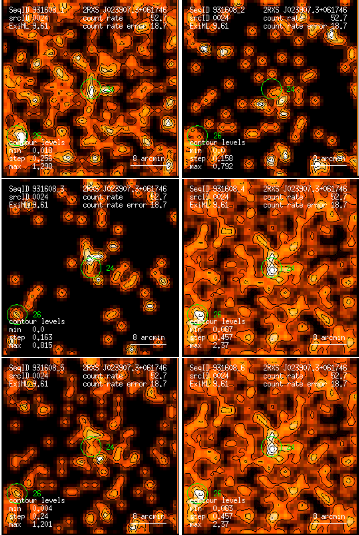
Figure 24: RASS 931608: detection 0024: band rate images, Gaussian filter: (1) PSPC channels 11 – 41, (2) 52 – 90, (3) 91 – 201, (4) 11 – 235, (5) 52 – 201, (6) 11 – 201. Broad band rates in counts/ks. Band rate contour levels in counts/ks/arcmin 2 .
