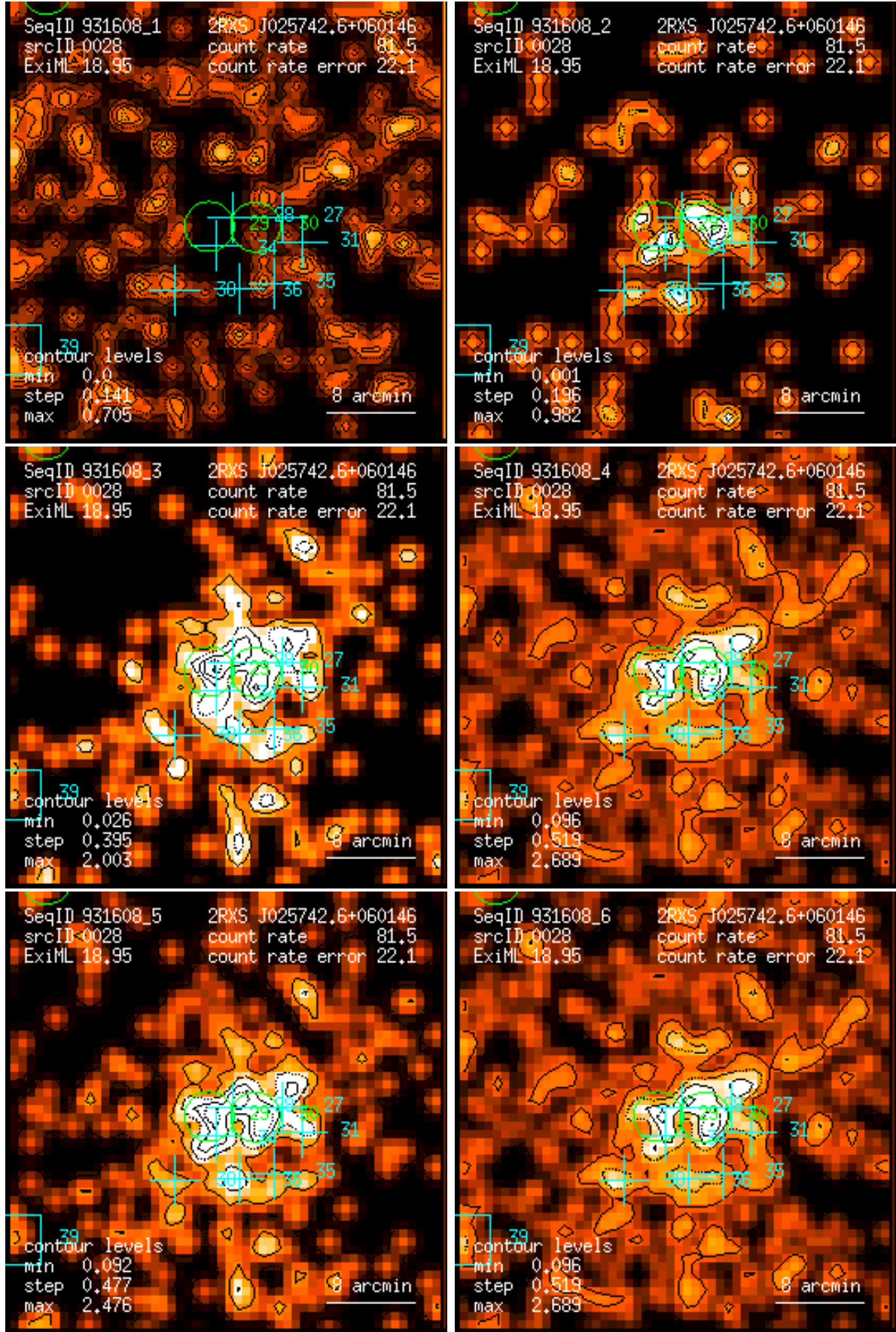
Figure 28: RASS 931608: detection 0028: band rate images, Gaussian filter: (1) PSPC channels 11 – 41, (2) 52 – 90, (3) 91 – 201, (4) 11 – 235, (5) 52 – 201, (6) 11 – 201. Broad band rates in counts/ks. Band rate contour levels in counts/ks/arcmin 2 .
