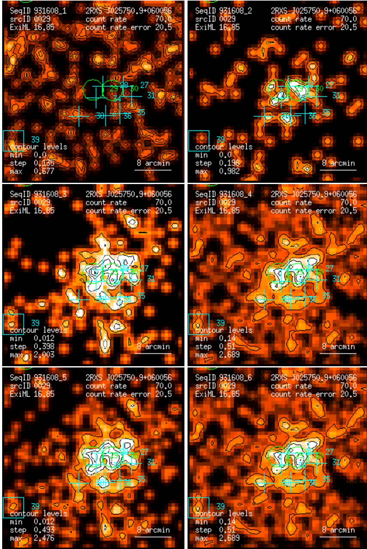
Figure 29: RASS 931608: detection 0029: band rate images, Gaussian filter: (1) PSPC channels 11 – 41, (2) 52 – 90, (3) 91 – 201, (4) 11 – 235, (5) 52 – 201, (6) 11 – 201. Broad band rates in counts/ks. Band rate contour levels in counts/ks/arcmin 2 .
