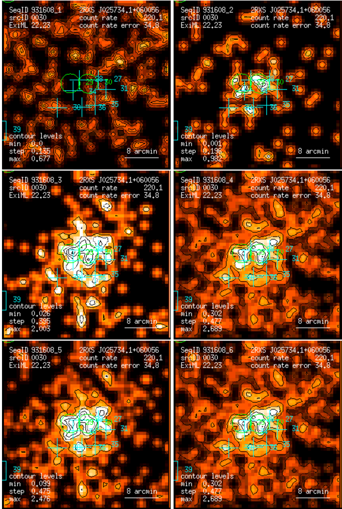
Figure 30: RASS 931608: detection 0030: band rate images, Gaussian filter: (1) PSPC channels 11 – 41, (2) 52 – 90, (3) 91 – 201, (4) 11 – 235, (5) 52 – 201, (6) 11 – 201. Broad band rates in counts/ks. Band rate contour levels in counts/ks/arcmin 2 .
