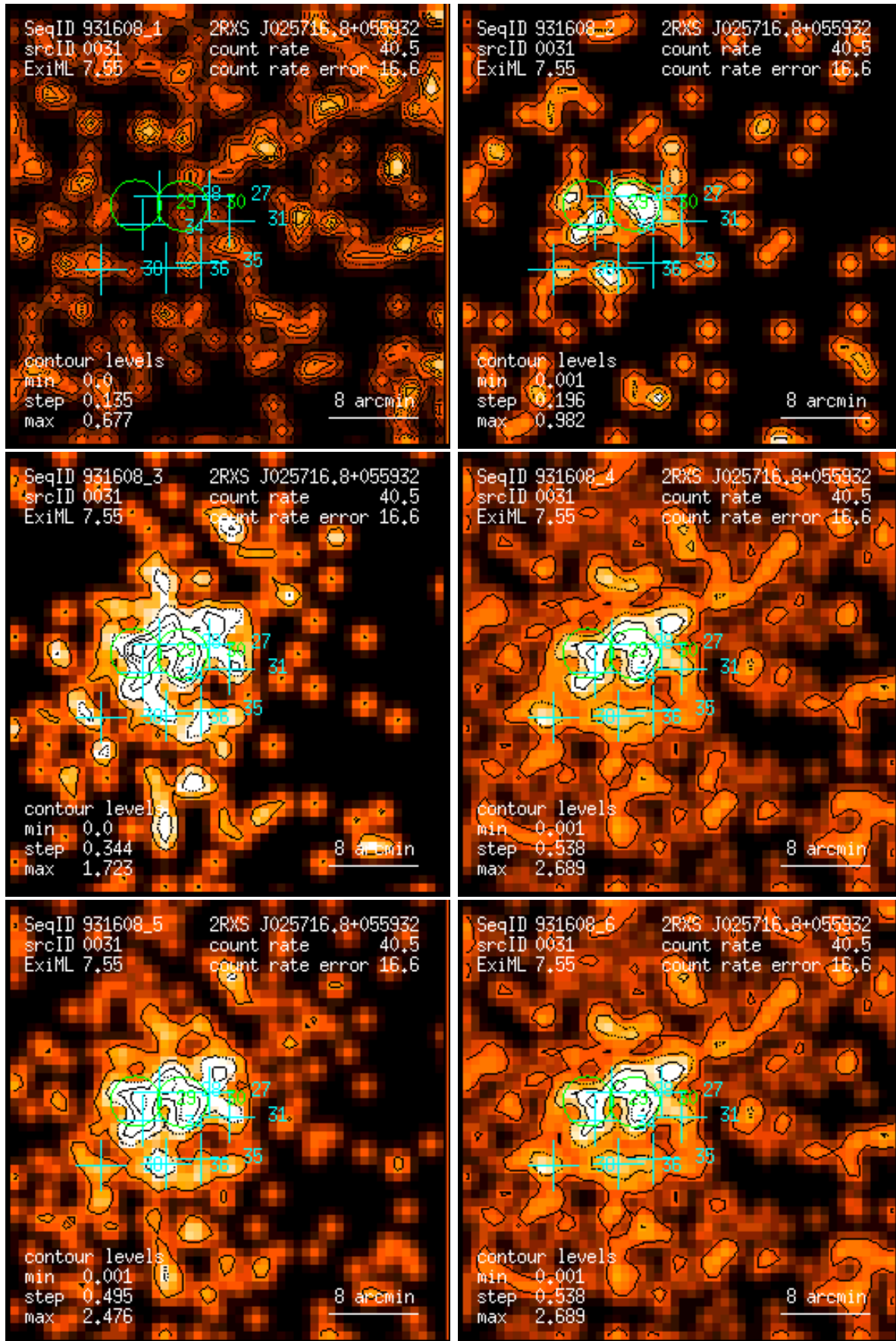
Figure 31: RASS 931608: detection 0031: band rate images, Gaussian filter: (1) PSPC channels 11 – 41, (2) 52 – 90, (3) 91 – 201, (4) 11 – 235, (5) 52 – 201, (6) 11 – 201. Broad band rates in counts/ks. Band rate contour levels in counts/ks/arcmin 2 .
