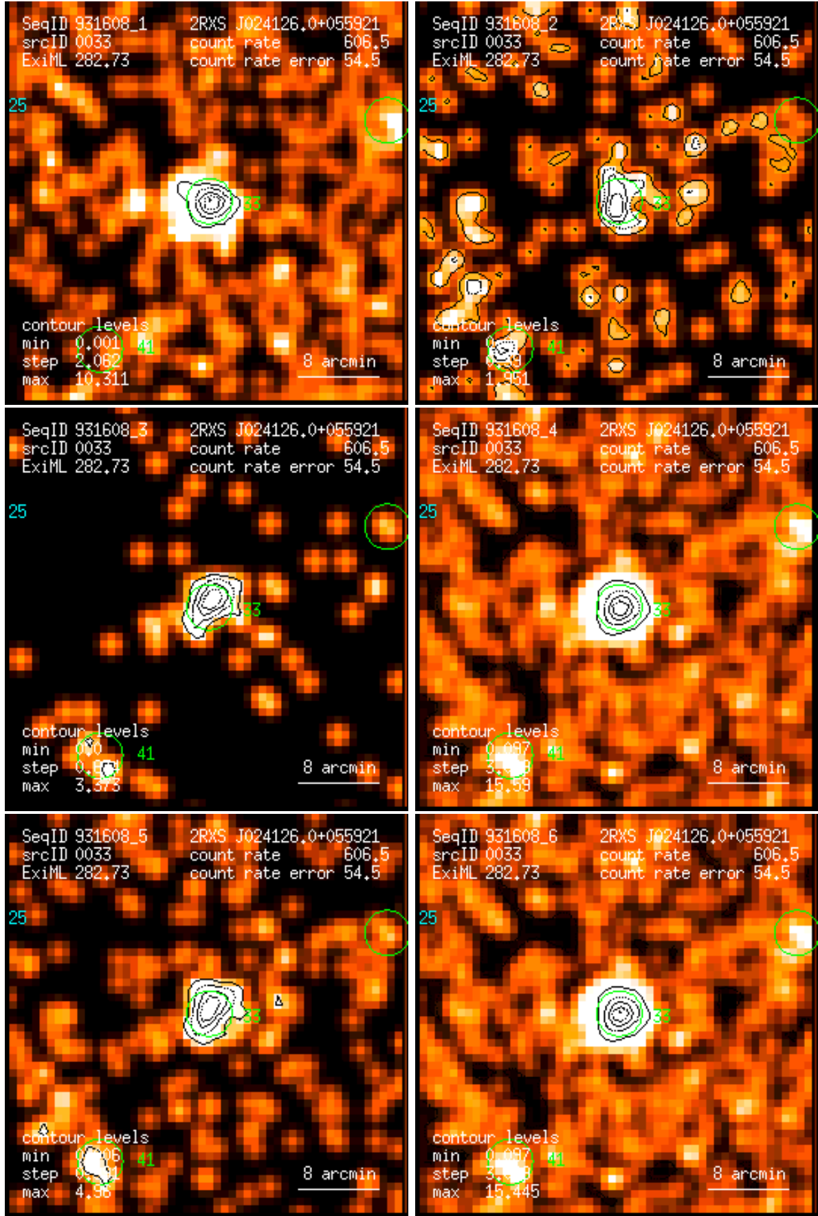
Figure 33: RASS 931608: detection 0033: band rate images, Gaussian filter: (1) PSPC channels 11 – 41, (2) 52 – 90, (3) 91 – 201, (4) 11 – 235, (5) 52 – 201, (6) 11 – 201. Broad band rates in counts/ks. Band rate contour levels in counts/ks/arcmin 2 .
