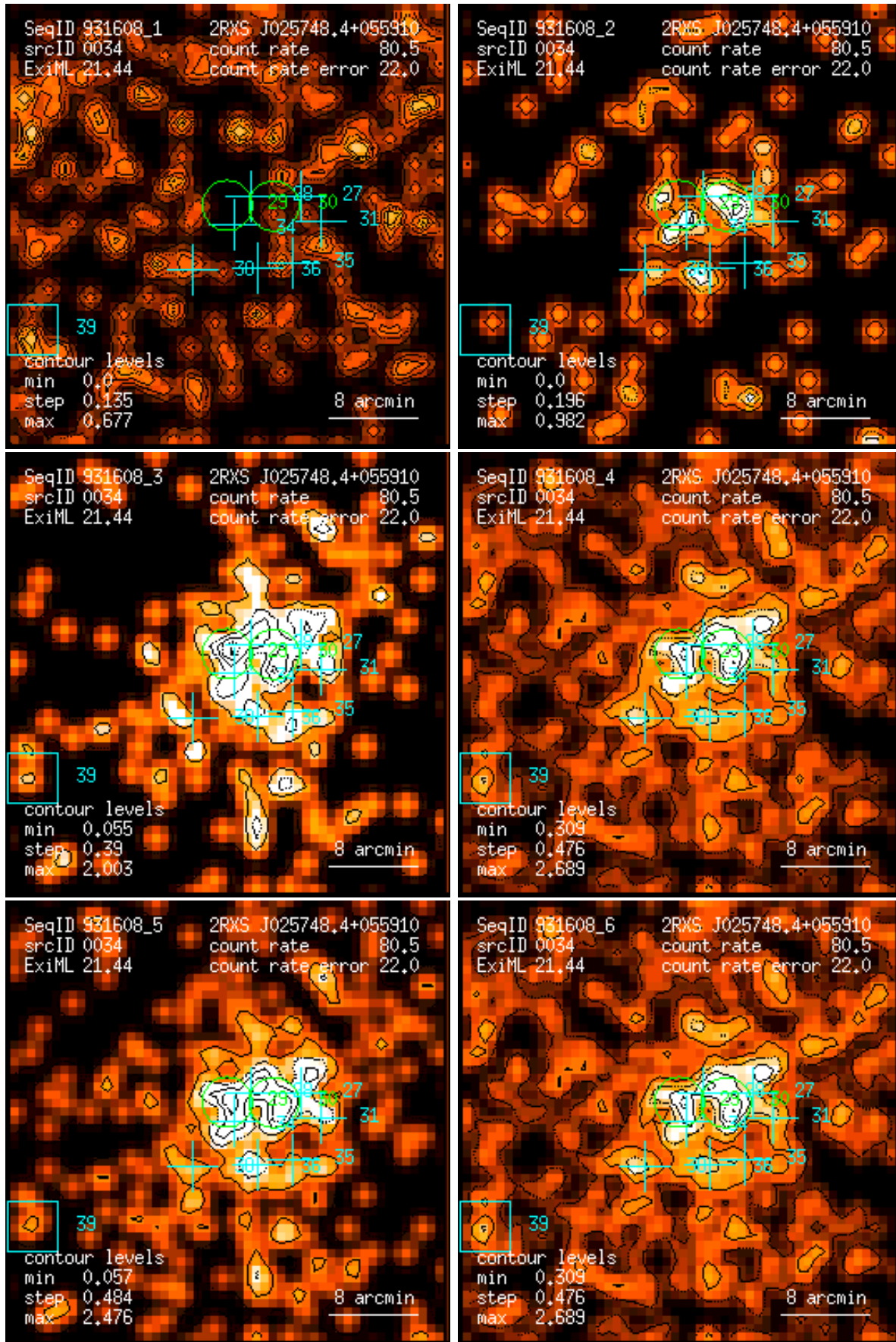
Figure 34: RASS 931608: detection 0034: band rate images, Gaussian filter: (1) PSPC channels 11 – 41, (2) 52 – 90, (3) 91 – 201, (4) 11 – 235, (5) 52 – 201, (6) 11 – 201. Broad band rates in counts/ks. Band rate contour levels in counts/ks/arcmin 2 .
