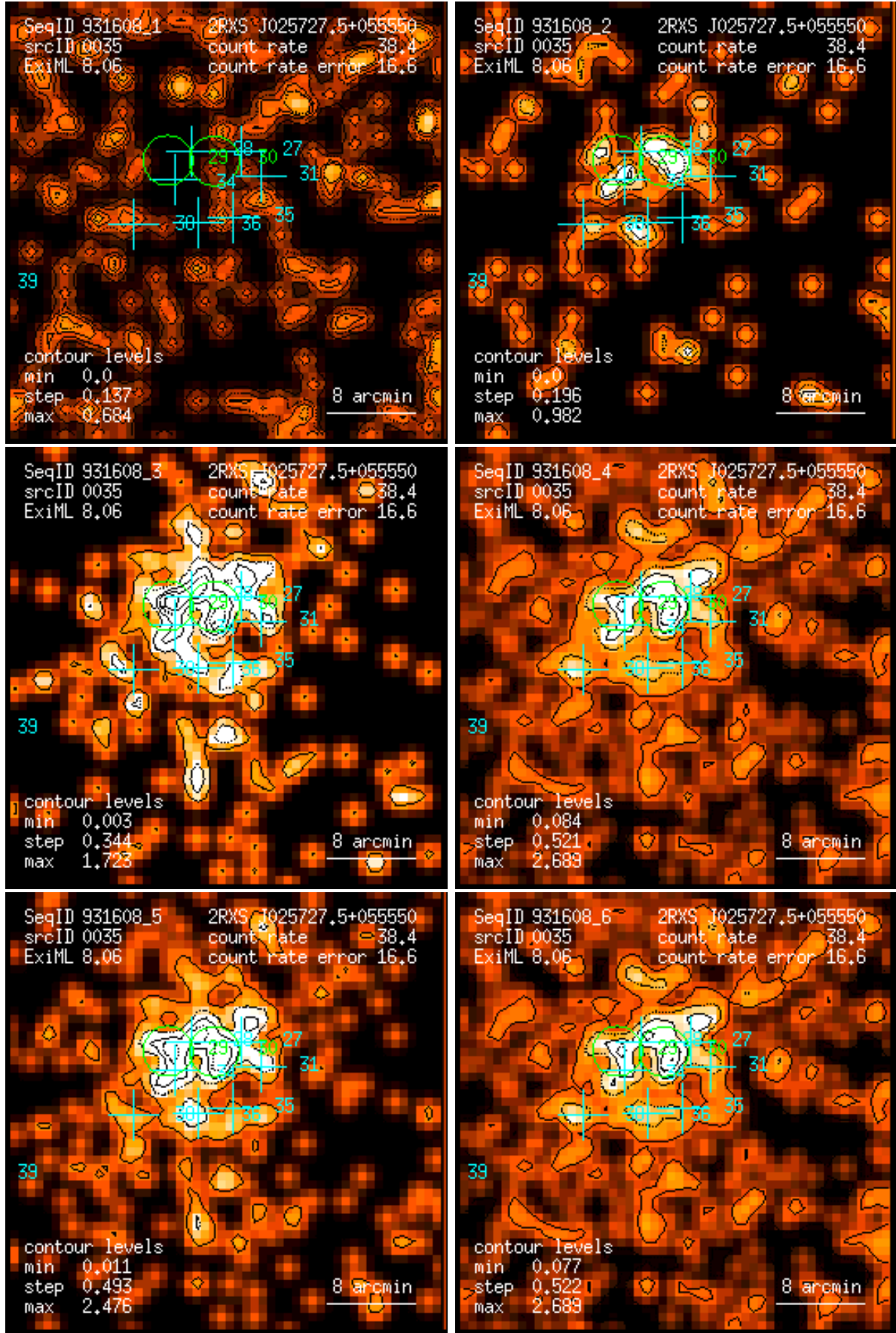
Figure 35: RASS 931608: detection 0035: band rate images, Gaussian filter: (1) PSPC channels 11 – 41, (2) 52 – 90, (3) 91 – 201, (4) 11 – 235, (5) 52 – 201, (6) 11 – 201. Broad band rates in counts/ks. Band rate contour levels in counts/ks/arcmin 2 .
