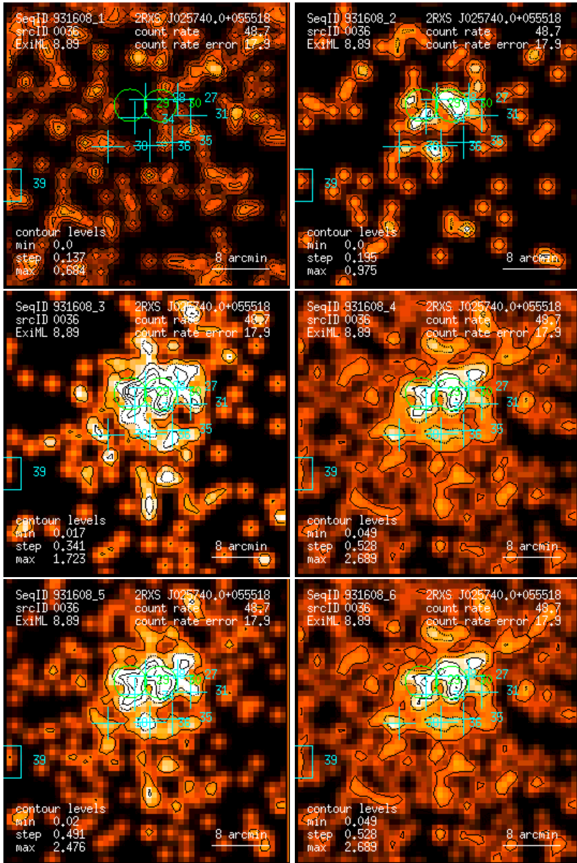
Figure 36: RASS 931608: detection 0036: band rate images, Gaussian filter: (1) PSPC channels 11 – 41, (2) 52 – 90, (3) 91 – 201, (4) 11 – 235, (5) 52 – 201, (6) 11 – 201. Broad band rates in counts/ks. Band rate contour levels in counts/ks/arcmin 2 .
