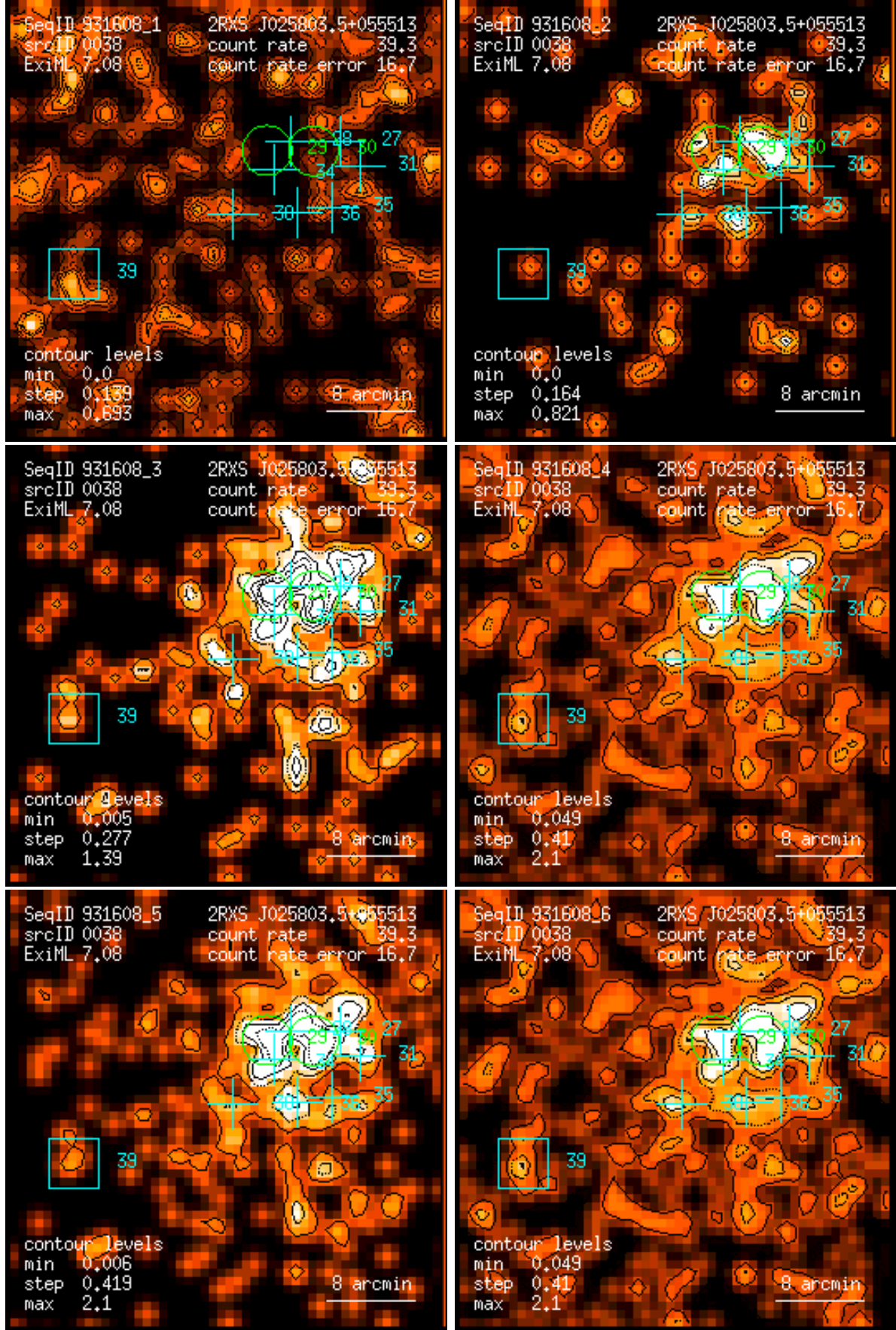
Figure 38: RASS 931608: detection 0038: band rate images, Gaussian filter: (1) PSPC channels 11 – 41, (2) 52 – 90, (3) 91 – 201, (4) 11 – 235, (5) 52 – 201, (6) 11 – 201. Broad band rates in counts/ks. Band rate contour levels in counts/ks/arcmin 2 .
