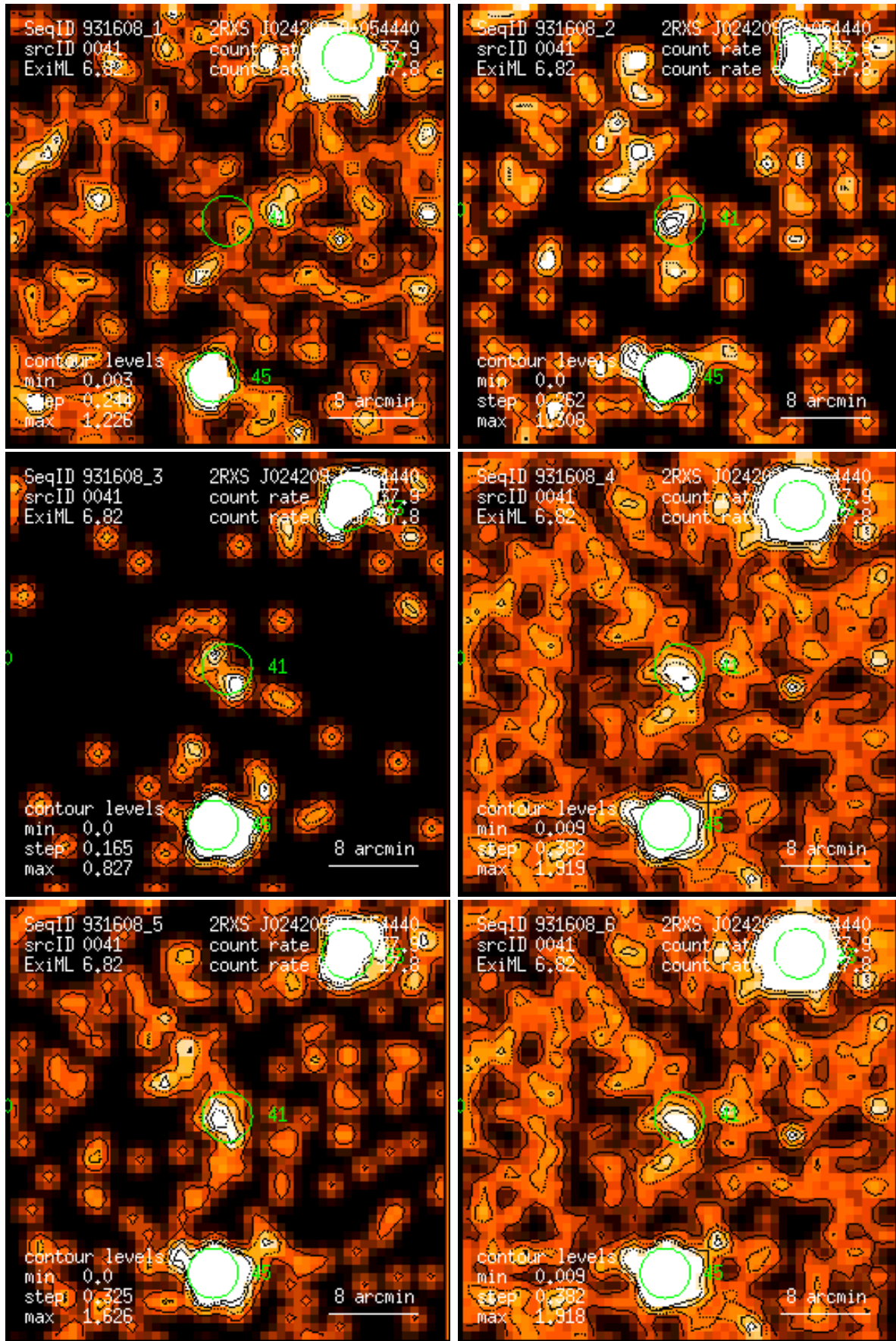
Figure 41: RASS 931608: detection 0041: band rate images, Gaussian filter: (1) PSPC channels 11 – 41, (2) 52 – 90, (3) 91 – 201, (4) 11 – 235, (5) 52 – 201, (6) 11 – 201. Broad band rates in counts/ks. Band rate contour levels in counts/ks/arcmin 2 .
