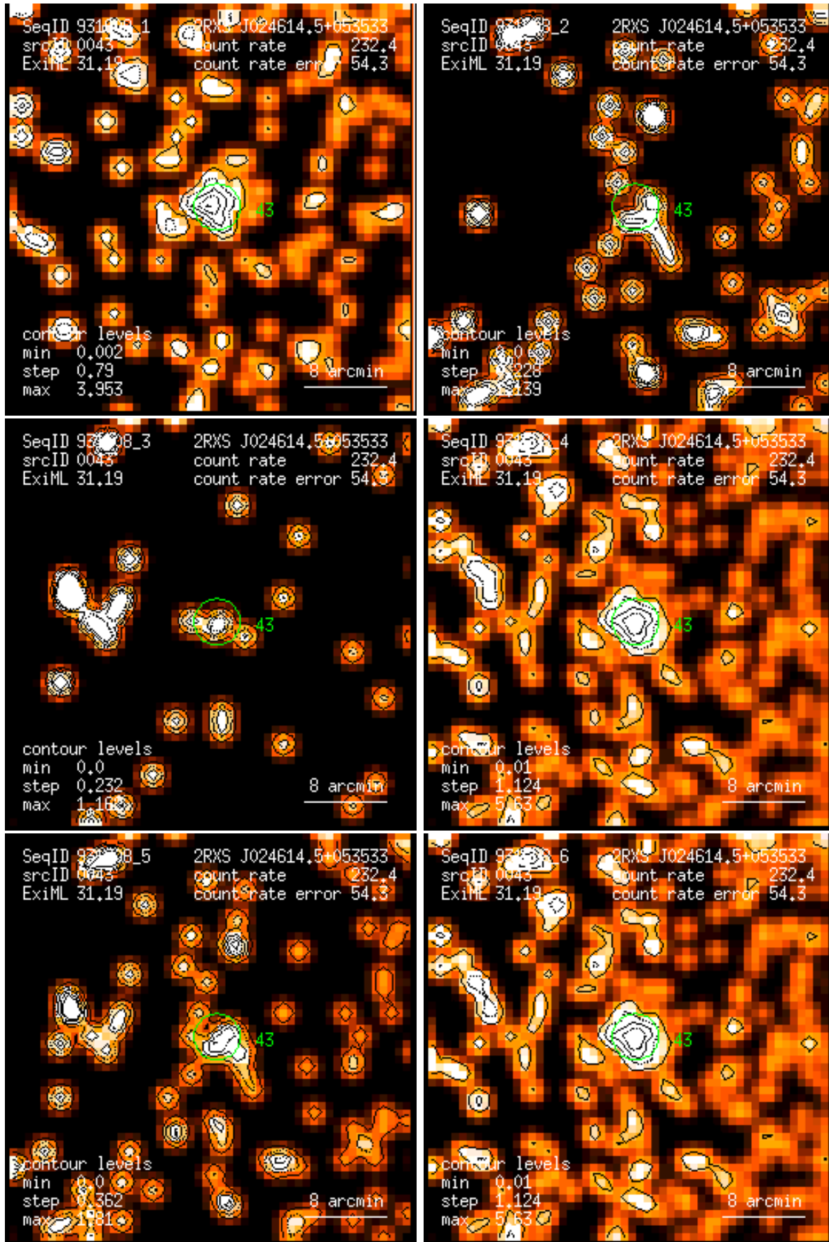
Figure 43: RASS 931608: detection 0043: band rate images, Gaussian filter: (1) PSPC channels 11 – 41, (2) 52 – 90, (3) 91 – 201, (4) 11 – 235, (5) 52 – 201, (6) 11 – 201. Broad band rates in counts/ks. Band rate contour levels in counts/ks/arcmin 2 .
