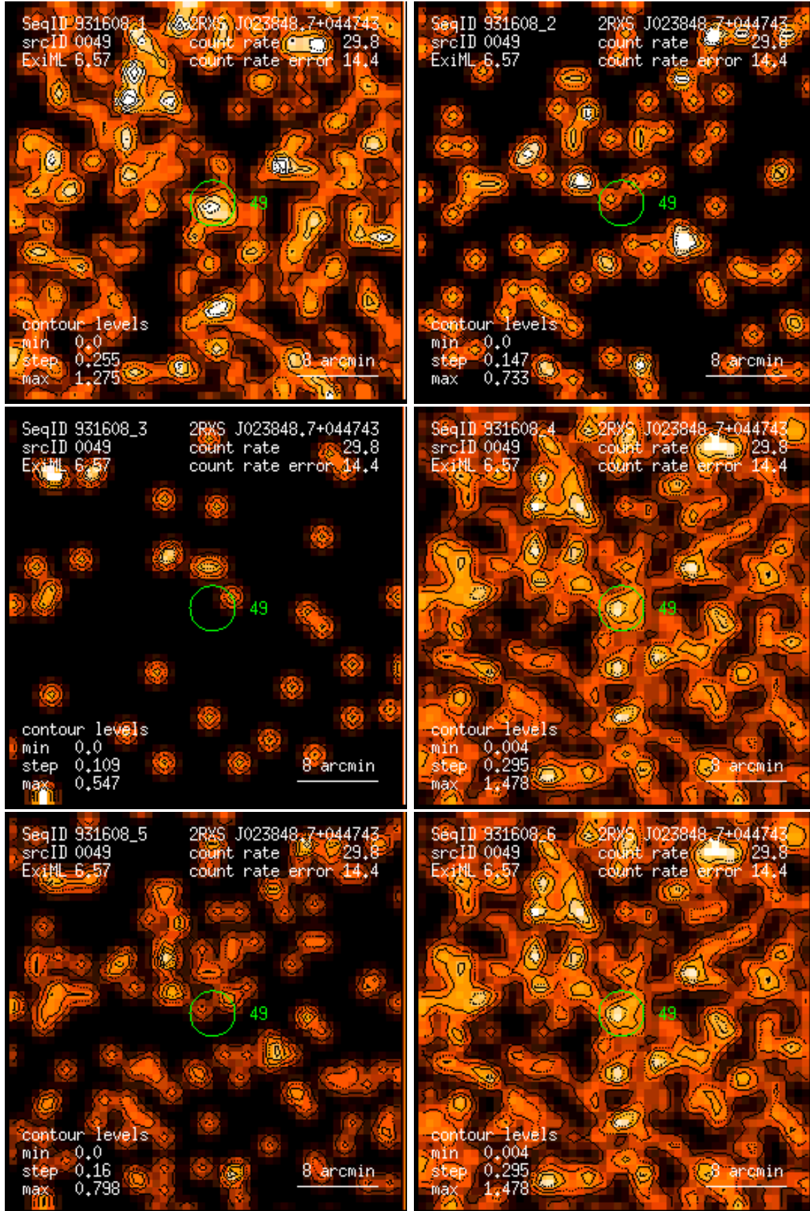
Figure 49: RASS 931608: detection 0049: band rate images, Gaussian filter: (1) PSPC channels 11 – 41, (2) 52 – 90, (3) 91 – 201, (4) 11 – 235, (5) 52 – 201, (6) 11 – 201. Broad band rates in counts/ks. Band rate contour levels in counts/ks/arcmin 2 .
