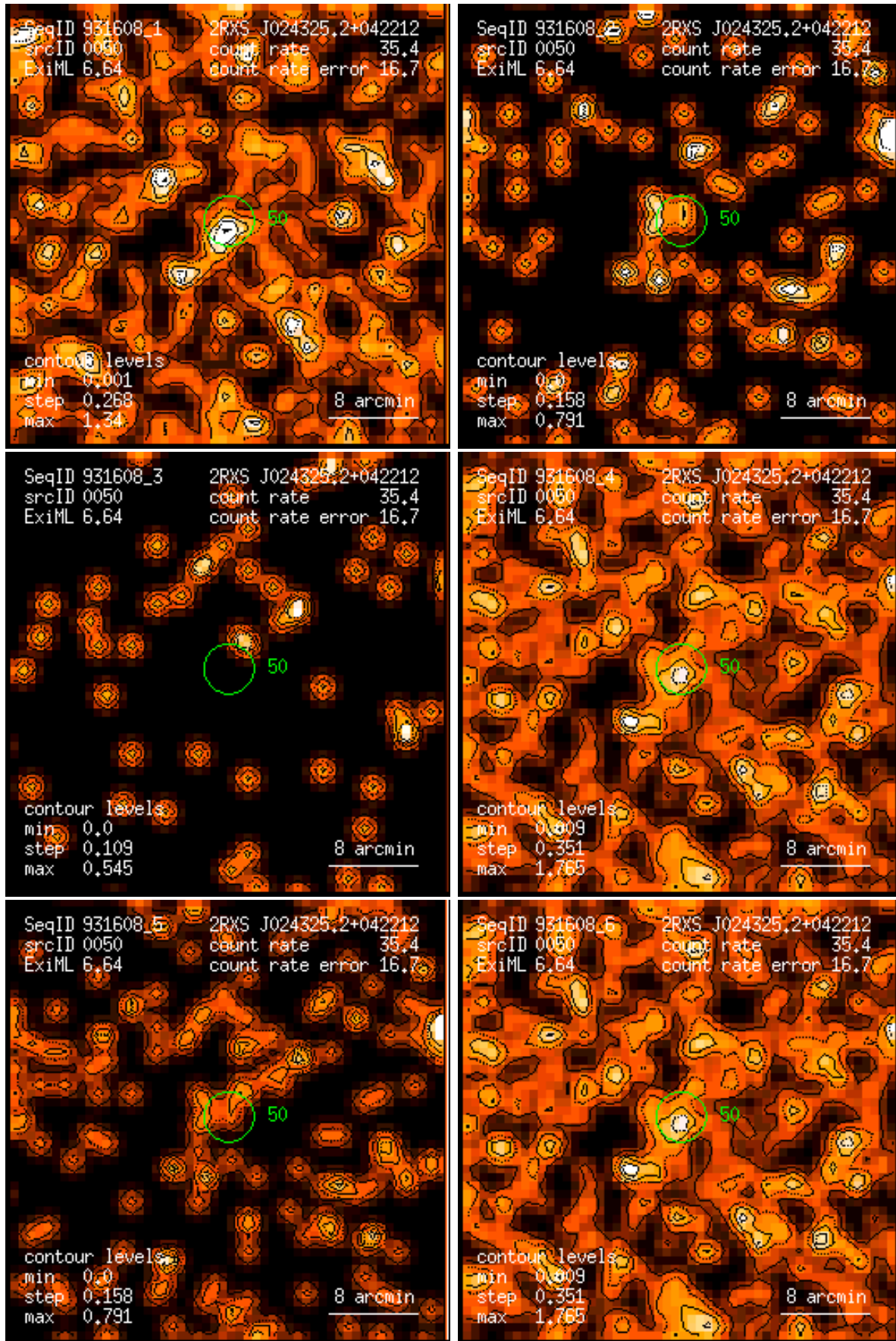
Figure 50: RASS 931608: detection 0050: band rate images, Gaussian filter: (1) PSPC channels 11 – 41, (2) 52 – 90, (3) 91 – 201, (4) 11 – 235, (5) 52 – 201, (6) 11 – 201. Broad band rates in counts/ks. Band rate contour levels in counts/ks/arcmin 2 .
