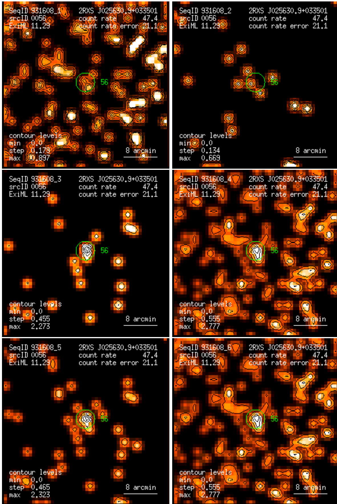
Figure 56: RASS 931608: detection 0056: band rate images, Gaussian filter: (1) PSPC channels 11 – 41, (2) 52 – 90, (3) 91 – 201, (4) 11 – 235, (5) 52 – 201, (6) 11 – 201. Broad band rates in counts/ks. Band rate contour levels in counts/ks/arcmin 2 .
