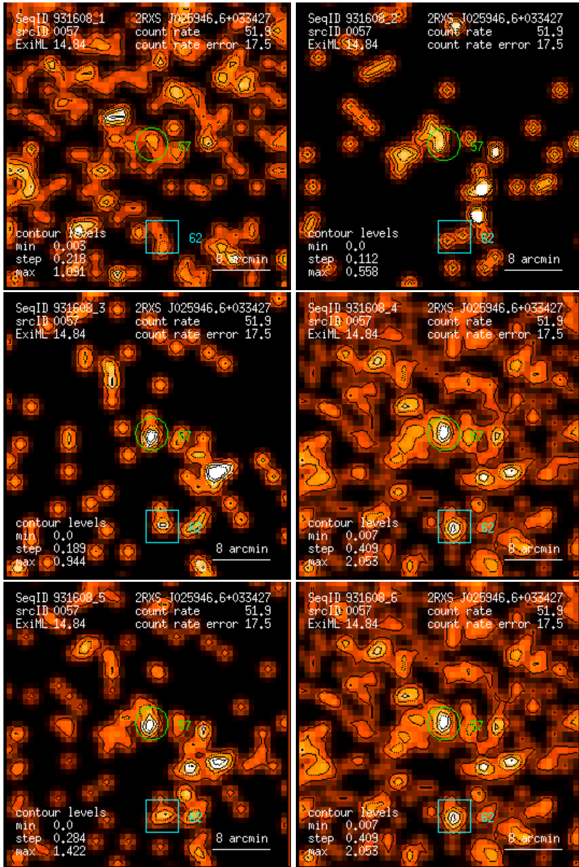
Figure 57: RASS 931608: detection 0057: band rate images, Gaussian filter: (1) PSPC channels 11 – 41, (2) 52 – 90, (3) 91 – 201, (4) 11 – 235, (5) 52 – 201, (6) 11 – 201. Broad band rates in counts/ks. Band rate contour levels in counts/ks/arcmin 2 .
