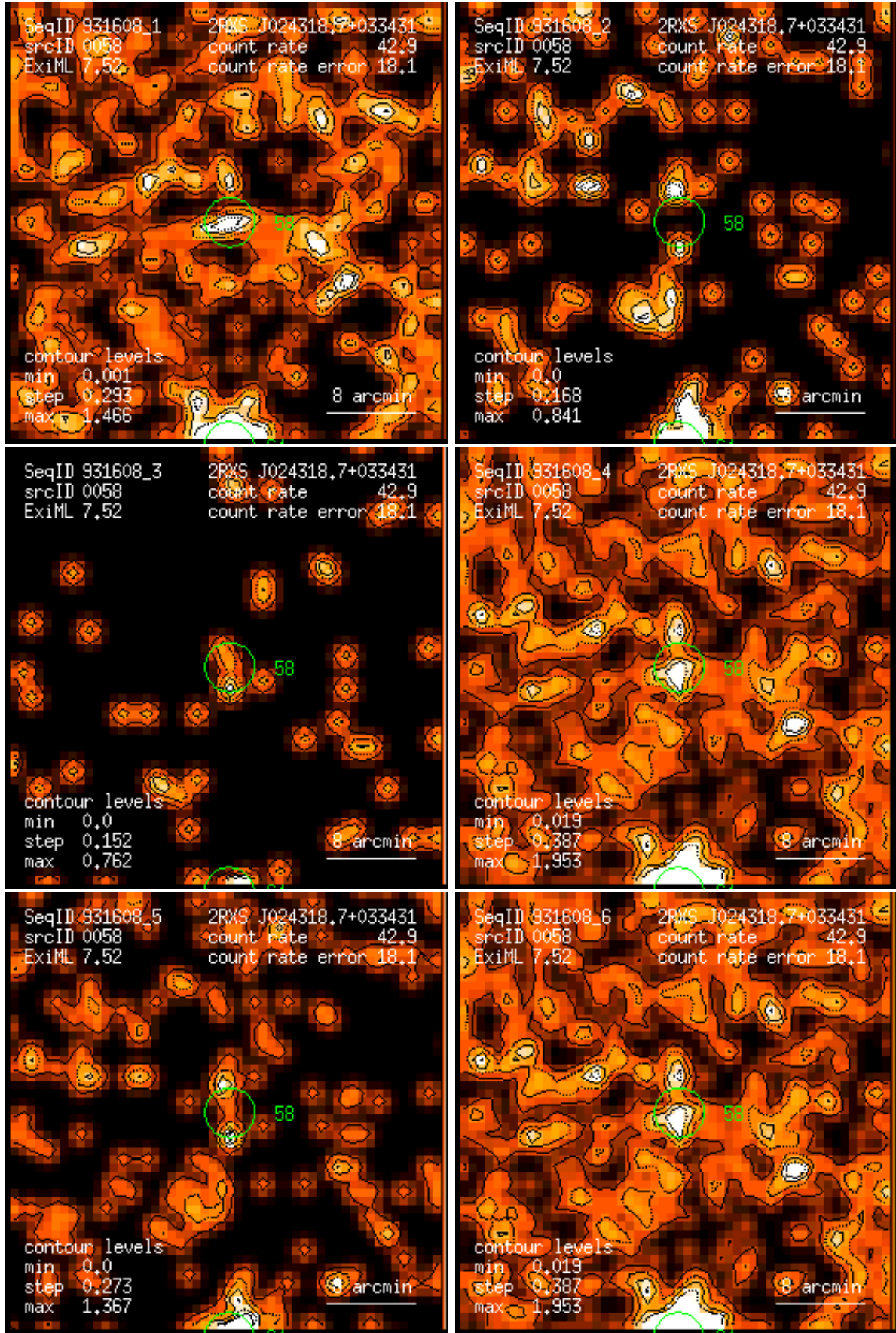
Figure 58: RASS 931608: detection 0058: band rate images, Gaussian filter: (1) PSPC channels 11 – 41, (2) 52 – 90, (3) 91 – 201, (4) 11 – 235, (5) 52 – 201, (6) 11 – 201. Broad band rates in counts/ks. Band rate contour levels in counts/ks/arcmin 2 .
