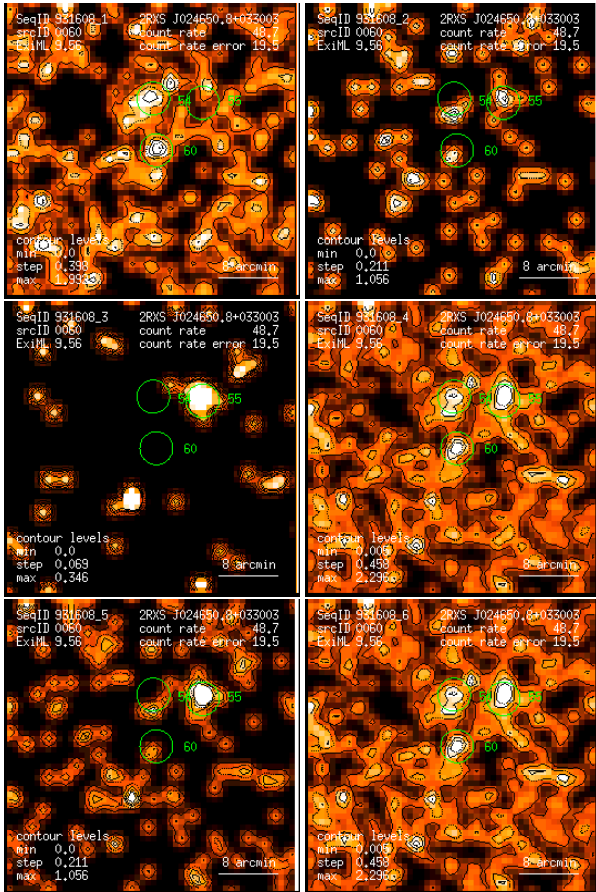
Figure 60: RASS 931608: detection 0060: band rate images, Gaussian filter: (1) PSPC channels 11 – 41, (2) 52 – 90, (3) 91 – 201, (4) 11 – 235, (5) 52 – 201, (6) 11 – 201. Broad band rates in counts/ks. Band rate contour levels in counts/ks/arcmin 2 .
