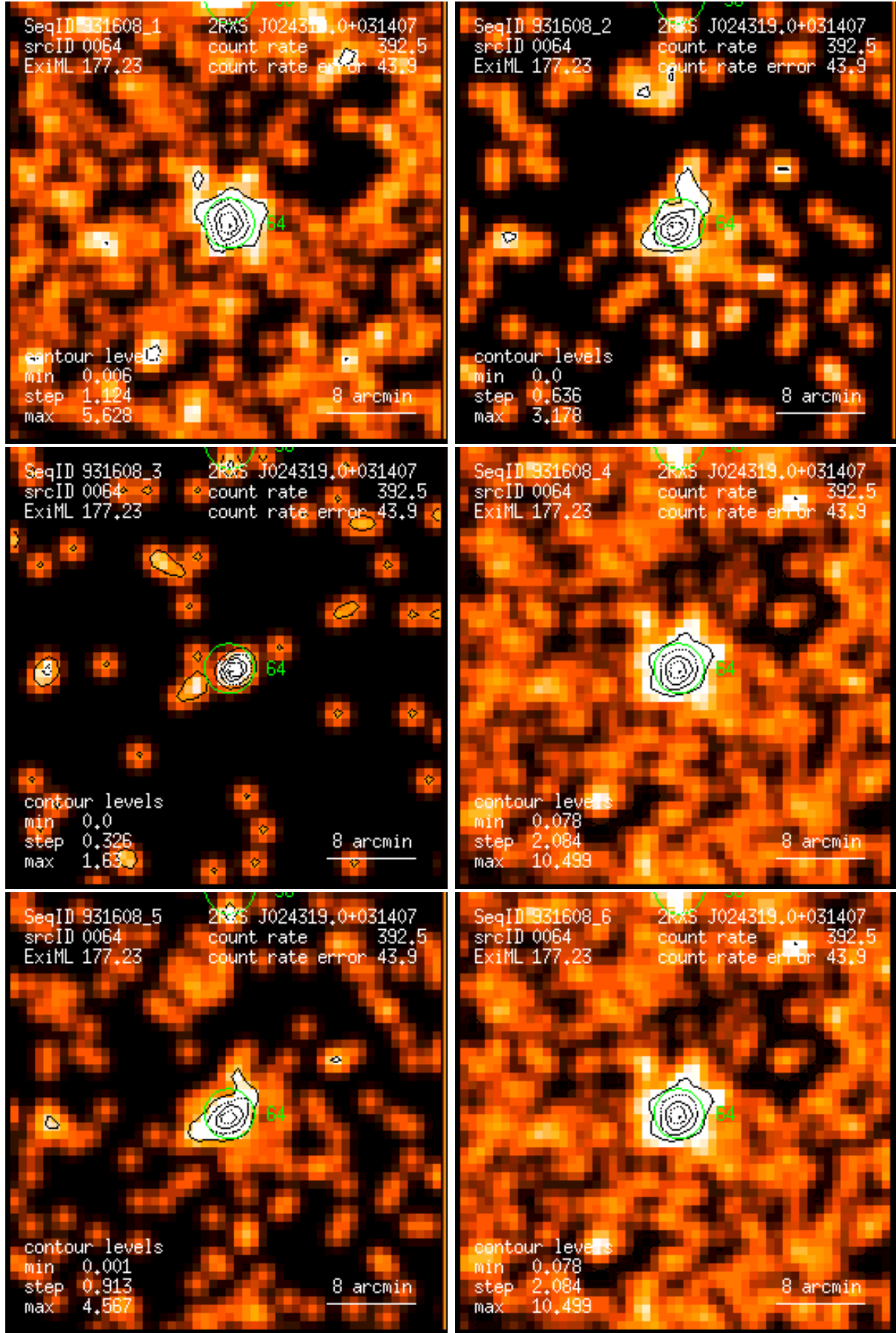
Figure 64: RASS 931608: detection 0064: band rate images, Gaussian filter: (1) PSPC channels 11 – 41, (2) 52 – 90, (3) 91 – 201, (4) 11 – 235, (5) 52 – 201, (6) 11 – 201. Broad band rates in counts/ks. Band rate contour levels in counts/ks/arcmin 2 .
