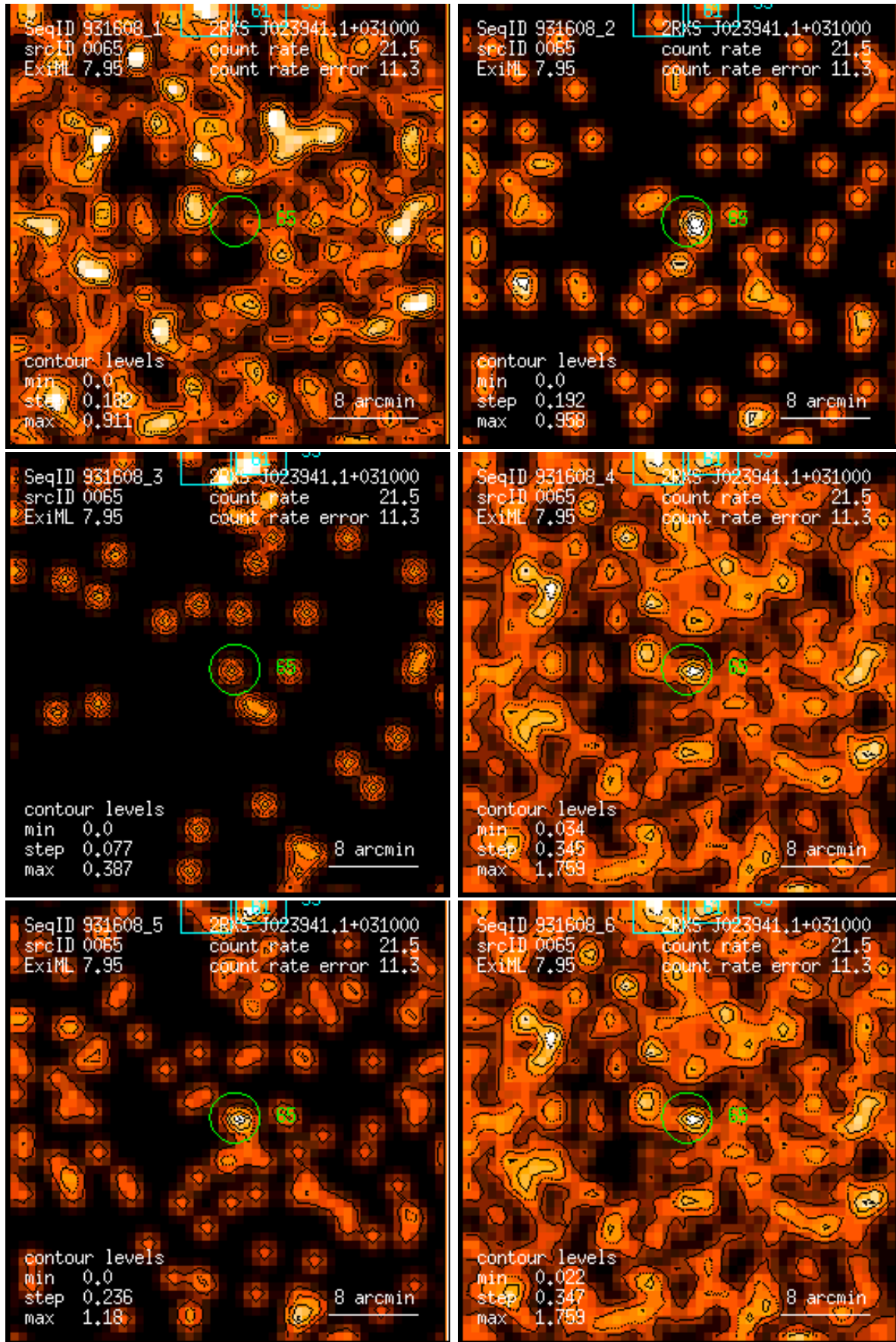
Figure 65: RASS 931608: detection 0065: band rate images, Gaussian filter: (1) PSPC channels 11 – 41, (2) 52 – 90, (3) 91 – 201, (4) 11 – 235, (5) 52 – 201, (6) 11 – 201. Broad band rates in counts/ks. Band rate contour levels in counts/ks/arcmin 2 .
