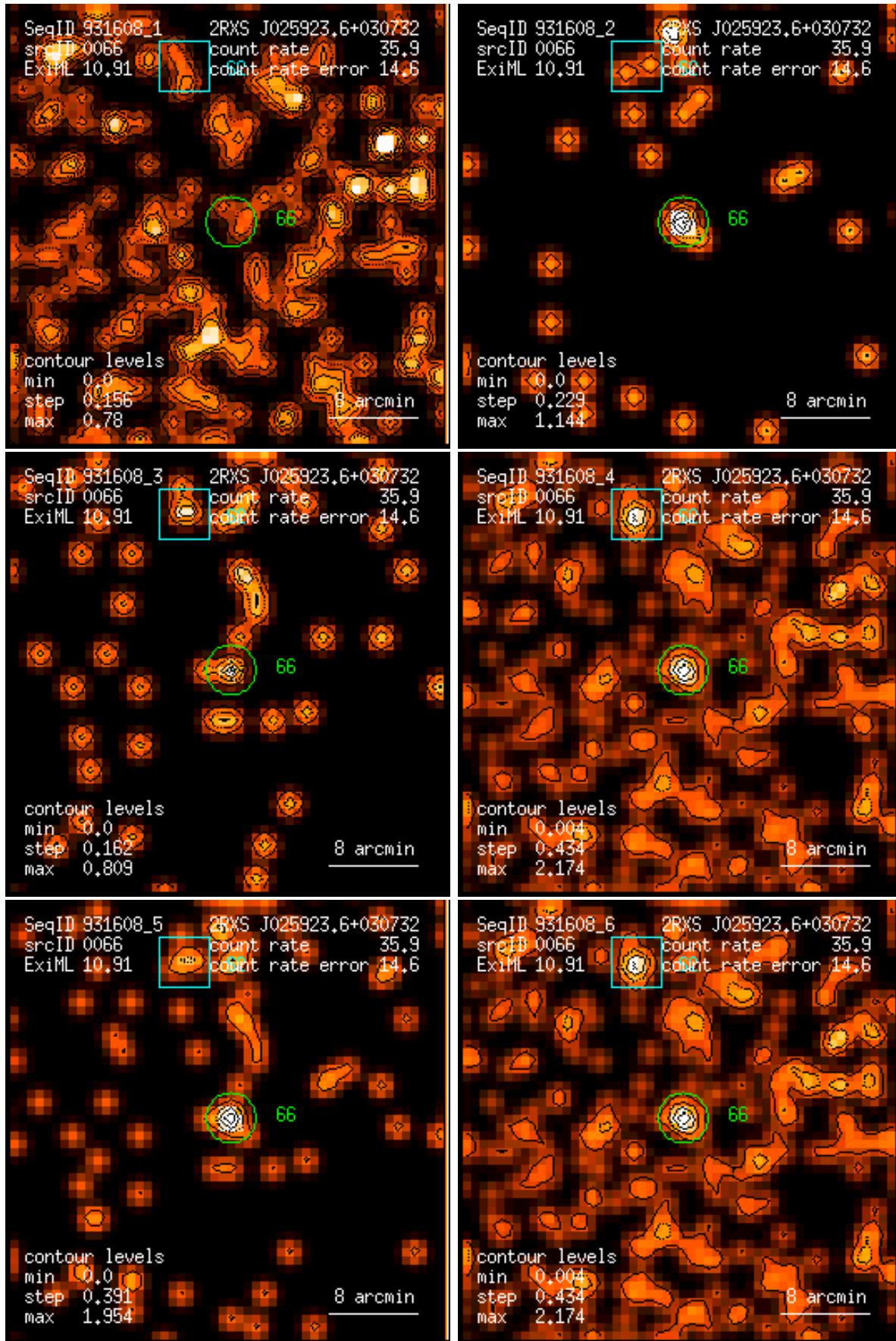
Figure 66: RASS 931608: detection 0066: band rate images, Gaussian filter: (1) PSPC channels 11 – 41, (2) 52 – 90, (3) 91 – 201, (4) 11 – 235, (5) 52 – 201, (6) 11 – 201. Broad band rates in counts/ks. Band rate contour levels in counts/ks/arcmin 2 .
