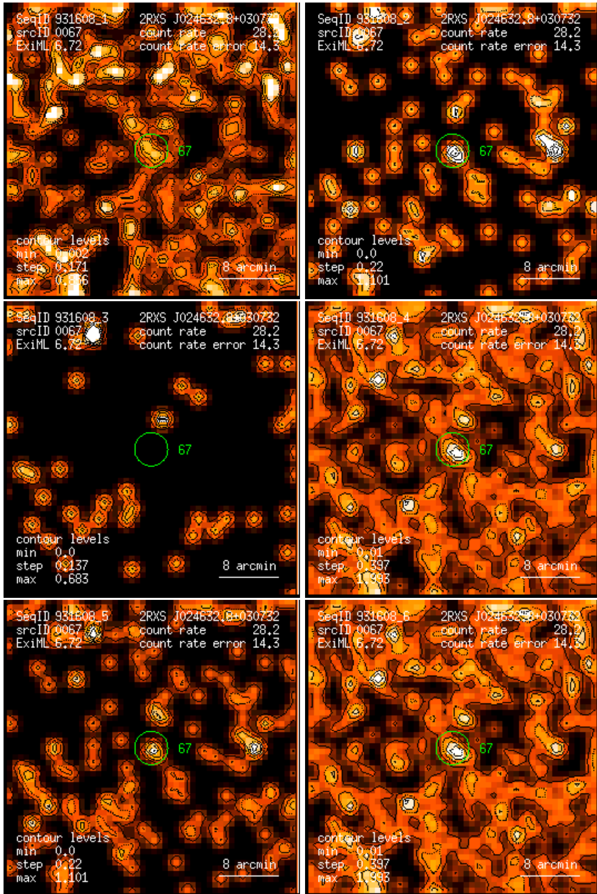
Figure 67: RASS 931608: detection 0067: band rate images, Gaussian filter: (1) PSPC channels 11 – 41, (2) 52 – 90, (3) 91 – 201, (4) 11 – 235, (5) 52 – 201, (6) 11 – 201. Broad band rates in counts/ks. Band rate contour levels in counts/ks/arcmin 2 .
