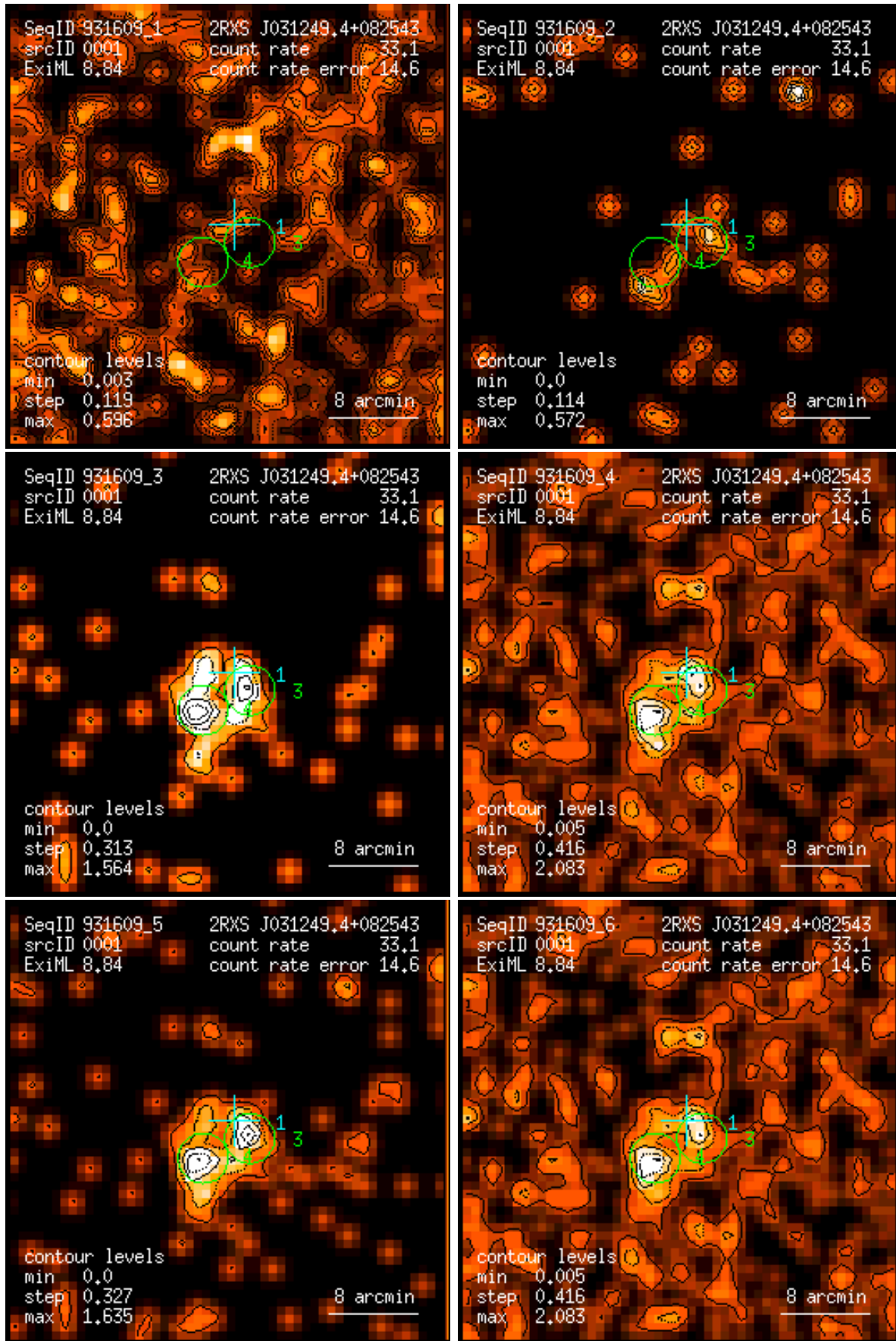
Figure 1: RASS 931609: detection 0001: band rate images, Gaussian filter: (1) PSPC channels 11 – 41, (2) 52 – 90, (3) 91 – 201, (4) 11 – 235, (5) 52 – 201, (6) 11 – 201. Broad band rates in counts/ks. Band rate contour levels in counts/ks/arcmin 2 .
