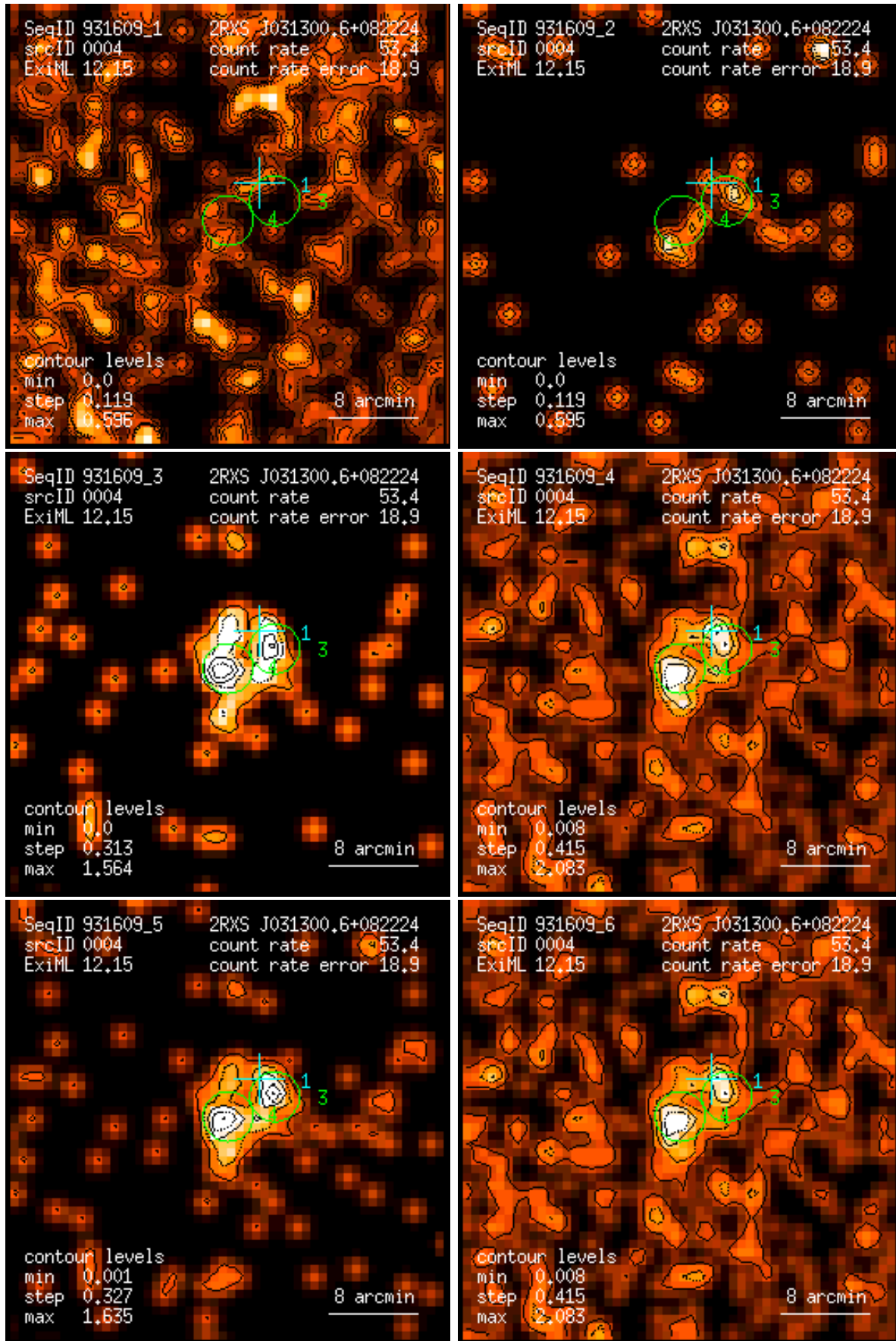
Figure 4: RASS 931609: detection 0004: band rate images, Gaussian filter: (1) PSPC channels 11 – 41, (2) 52 – 90, (3) 91 – 201, (4) 11 – 235, (5) 52 – 201, (6) 11 – 201. Broad band rates in counts/ks. Band rate contour levels in counts/ks/arcmin 2 .
