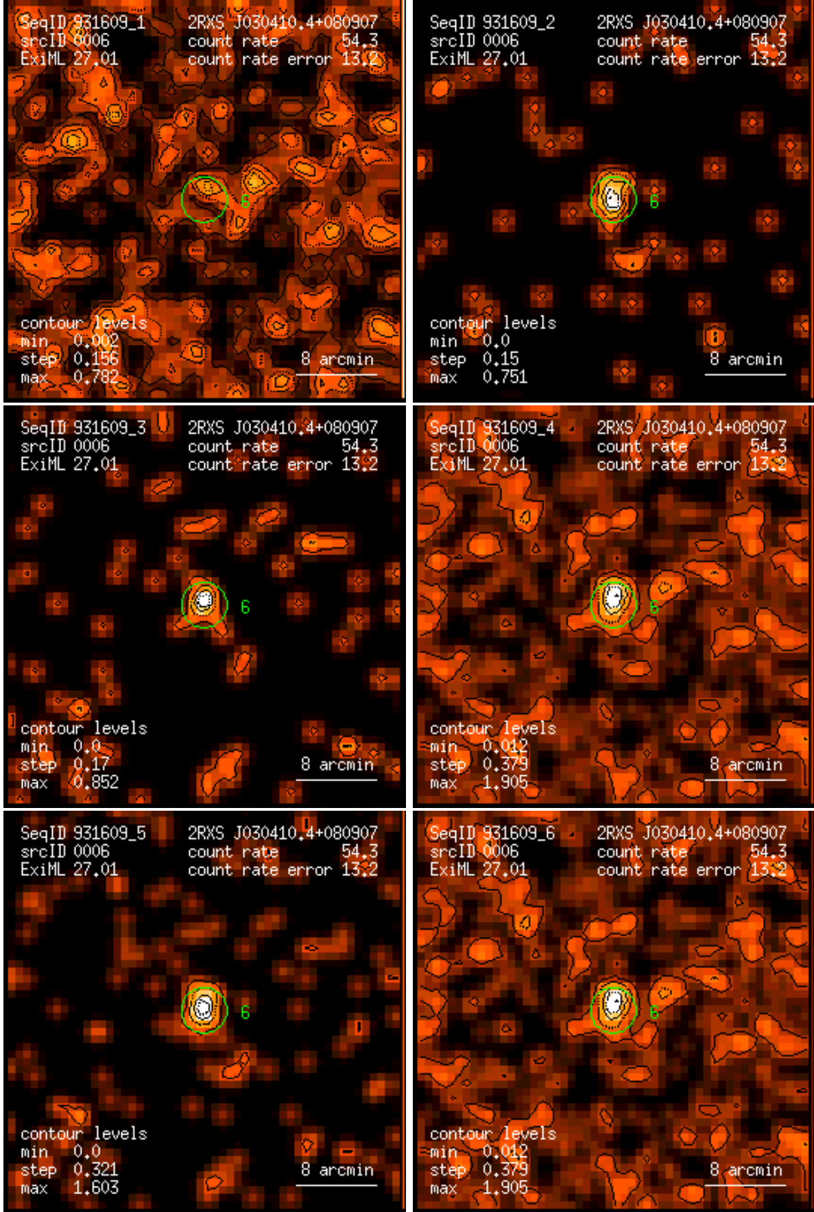
Figure 6: RASS 931609: detection 0006: band rate images, Gaussian filter: (1) PSPC channels 11 – 41, (2) 52 – 90, (3) 91 – 201, (4) 11 – 235, (5) 52 – 201, (6) 11 – 201. Broad band rates in counts/ks. Band rate contour levels in counts/ks/arcmin 2 .
