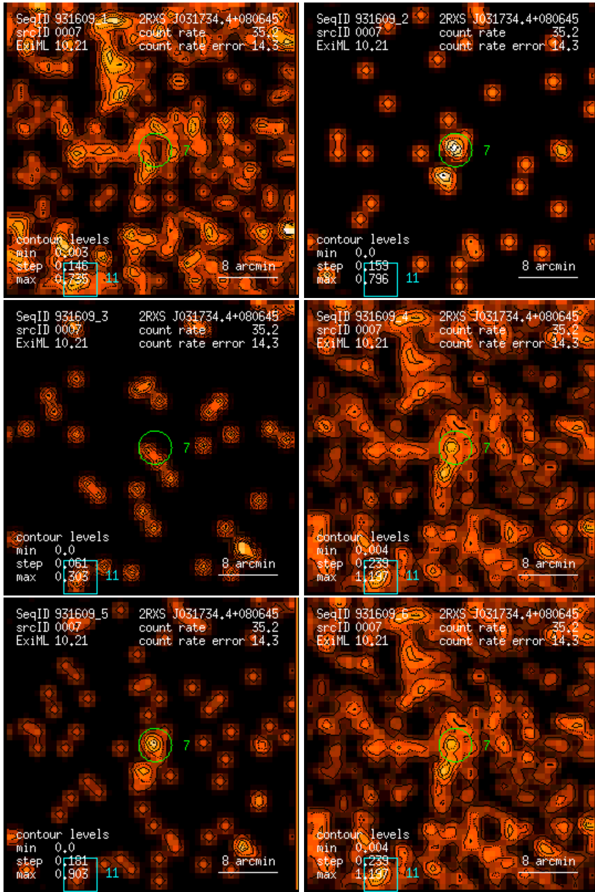
Figure 7: RASS 931609: detection 0007: band rate images, Gaussian filter: (1) PSPC channels 11 – 41, (2) 52 – 90, (3) 91 – 201, (4) 11 – 235, (5) 52 – 201, (6) 11 – 201. Broad band rates in counts/ks. Band rate contour levels in counts/ks/arcmin 2 .
