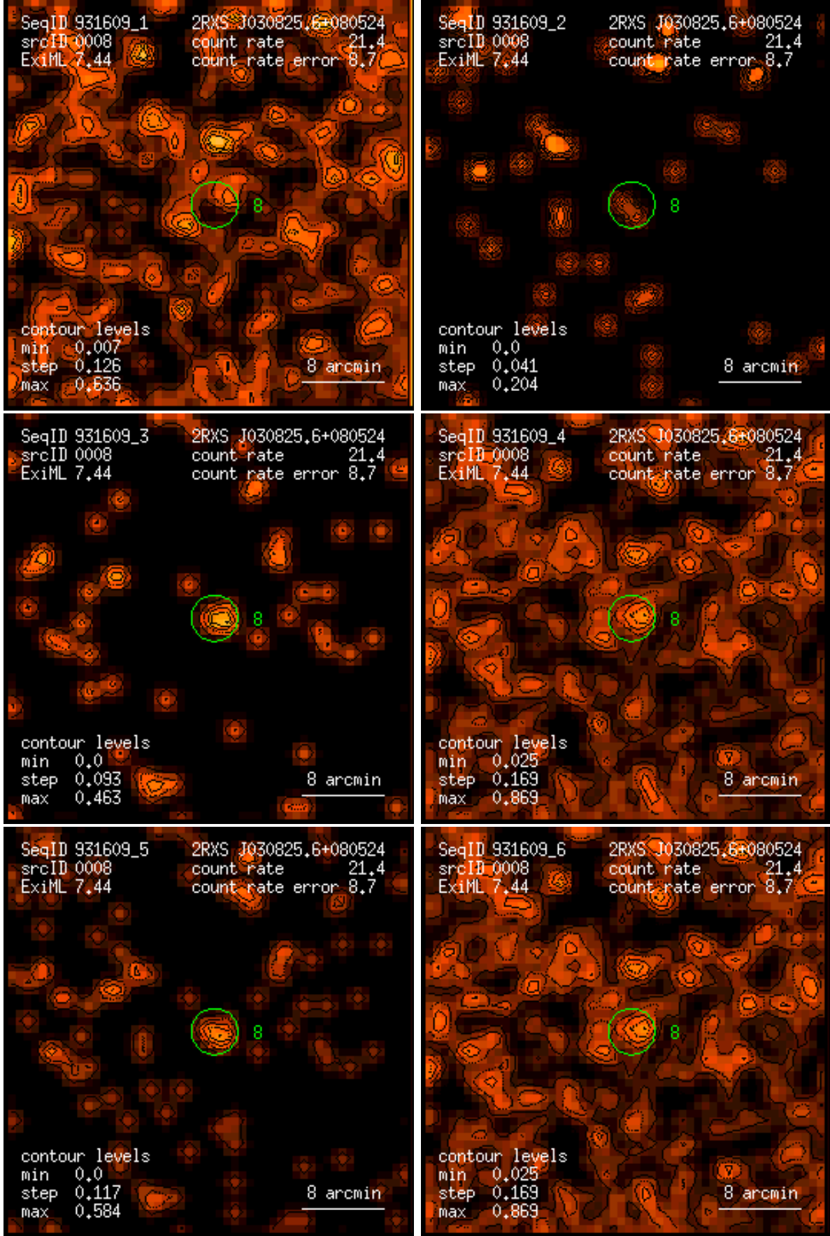
Figure 8: RASS 931609: detection 0008: band rate images, Gaussian filter: (1) PSPC channels 11 – 41, (2) 52 – 90, (3) 91 – 201, (4) 11 – 235, (5) 52 – 201, (6) 11 – 201. Broad band rates in counts/ks. Band rate contour levels in counts/ks/arcmin 2 .
