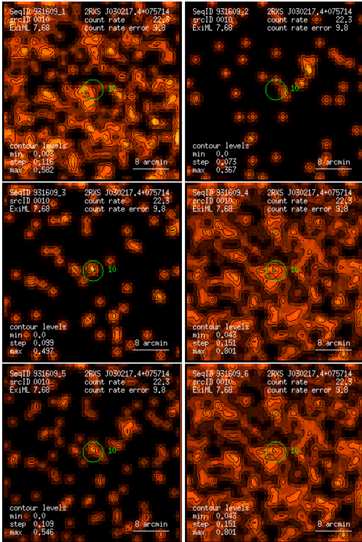
Figure 10: RASS 931609: detection 0010: band rate images, Gaussian filter: (1) PSPC channels 11 – 41, (2) 52 – 90, (3) 91 – 201, (4) 11 – 235, (5) 52 – 201, (6) 11 – 201. Broad band rates in counts/ks. Band rate contour levels in counts/ks/arcmin 2 .
