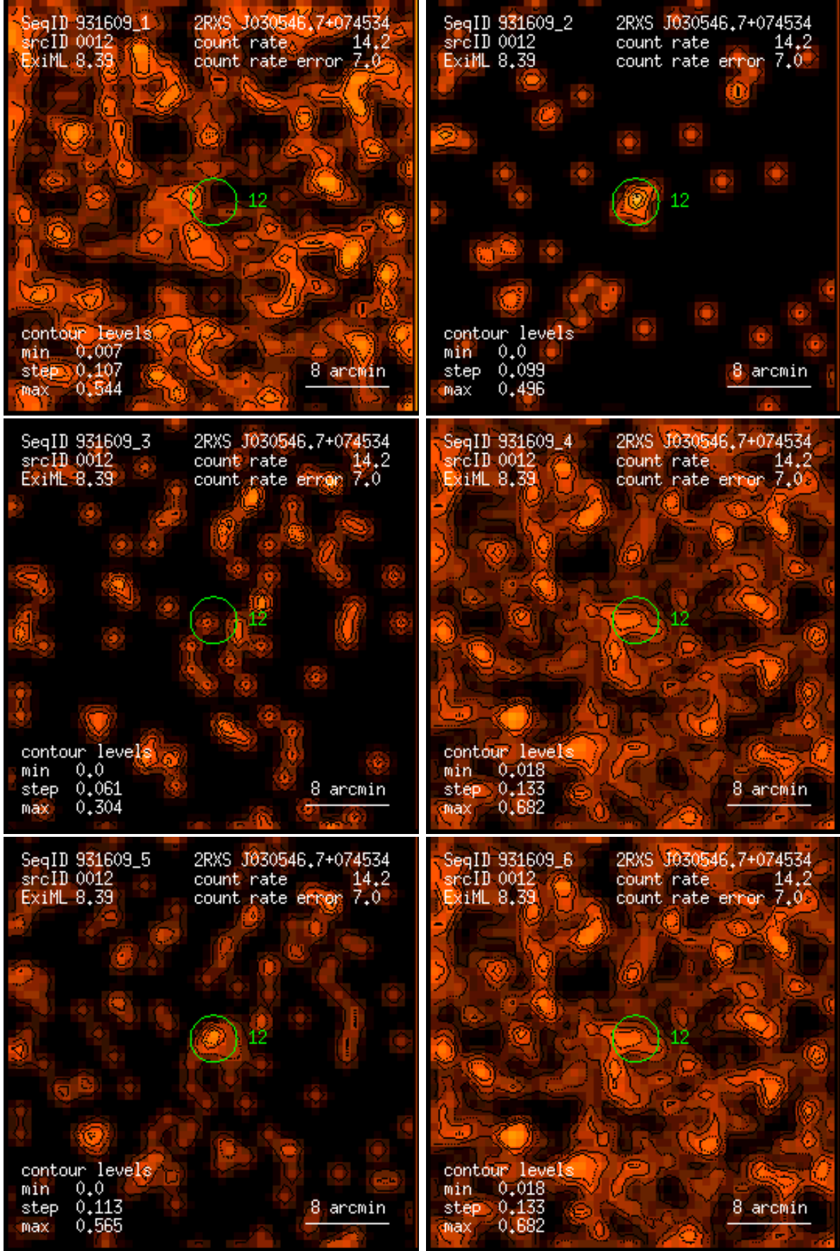
Figure 12: RASS 931609: detection 0012: band rate images, Gaussian filter: (1) PSPC channels 11 – 41, (2) 52 – 90, (3) 91 – 201, (4) 11 – 235, (5) 52 – 201, (6) 11 – 201. Broad band rates in counts/ks. Band rate contour levels in counts/ks/arcmin 2 .
