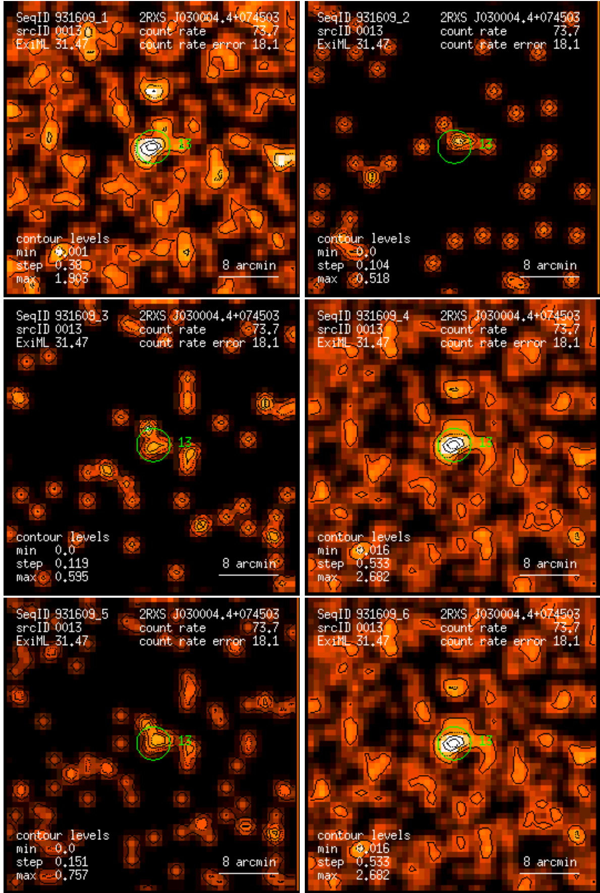
Figure 13: RASS 931609: detection 0013: band rate images, Gaussian filter: (1) PSPC channels 11 – 41, (2) 52 – 90, (3) 91 – 201, (4) 11 – 235, (5) 52 – 201, (6) 11 – 201. Broad band rates in counts/ks. Band rate contour levels in counts/ks/arcmin 2 .
