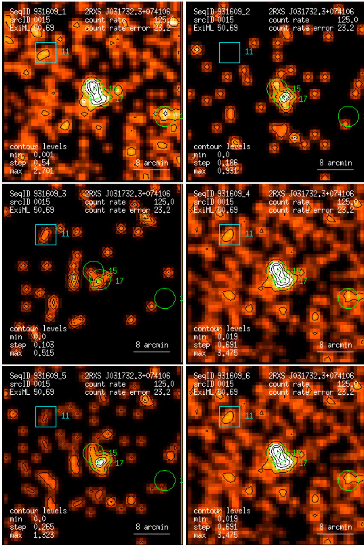
Figure 15: RASS 931609: detection 0015: band rate images, Gaussian filter: (1) PSPC channels 11 – 41, (2) 52 – 90, (3) 91 – 201, (4) 11 – 235, (5) 52 – 201, (6) 11 – 201. Broad band rates in counts/ks. Band rate contour levels in counts/ks/arcmin 2 .
