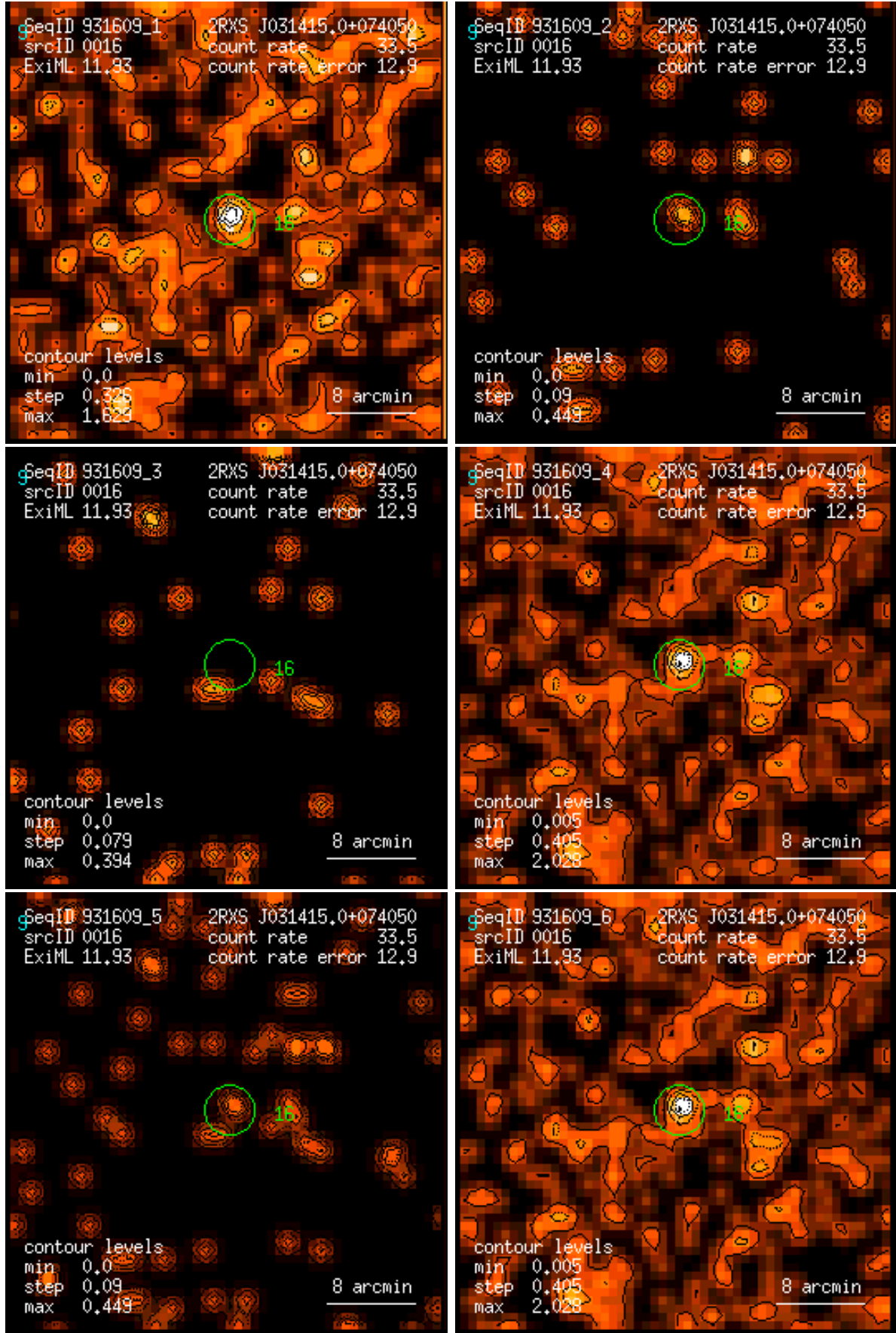
Figure 16: RASS 931609: detection 0016: band rate images, Gaussian filter: (1) PSPC channels 11 – 41, (2) 52 – 90, (3) 91 – 201, (4) 11 – 235, (5) 52 – 201, (6) 11 – 201. Broad band rates in counts/ks. Band rate contour levels in counts/ks/arcmin 2 .
