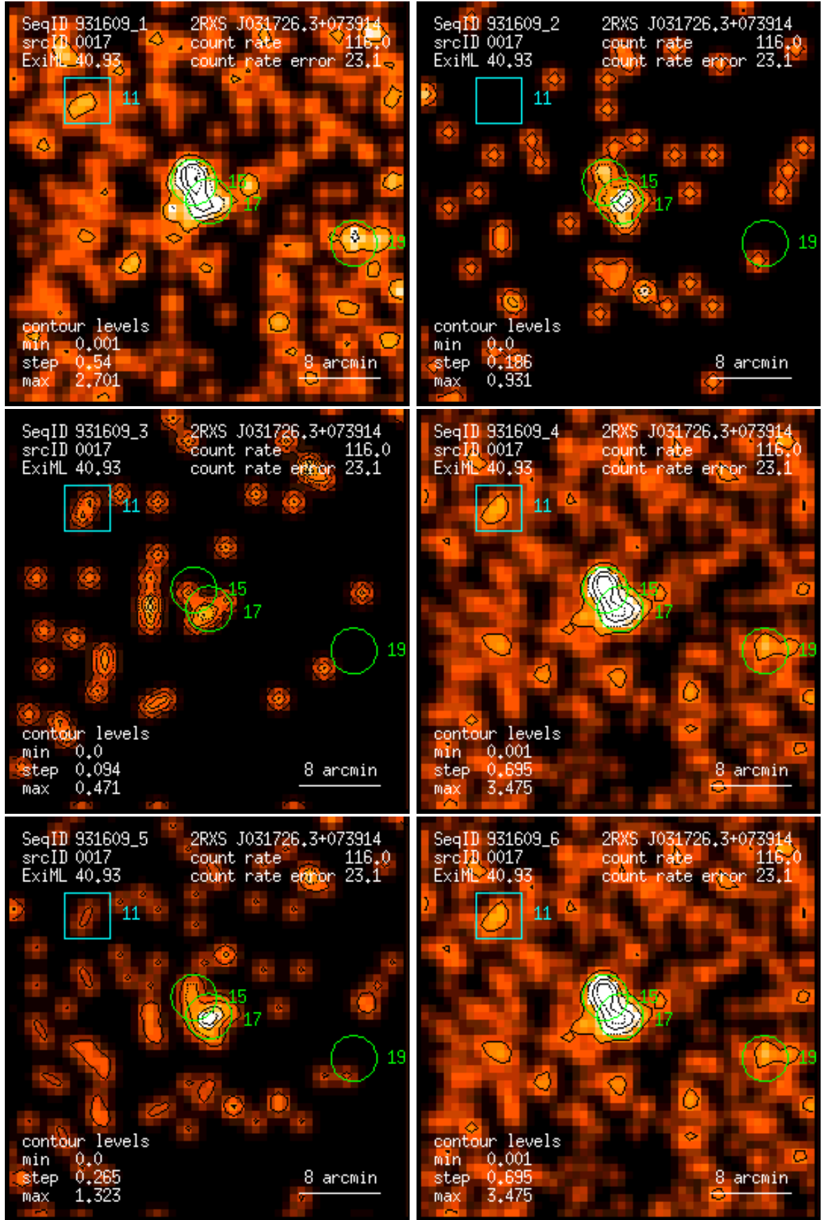
Figure 17: RASS 931609: detection 0017: band rate images, Gaussian filter: (1) PSPC channels 11 – 41, (2) 52 – 90, (3) 91 – 201, (4) 11 – 235, (5) 52 – 201, (6) 11 – 201. Broad band rates in counts/ks. Band rate contour levels in counts/ks/arcmin 2 .
