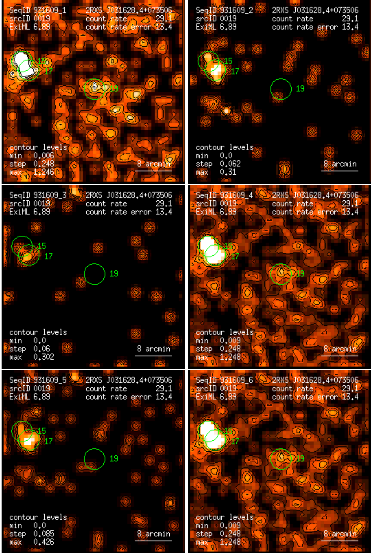
Figure 19: RASS 931609: detection 0019: band rate images, Gaussian filter: (1) PSPC channels 11 – 41, (2) 52 – 90, (3) 91 – 201, (4) 11 – 235, (5) 52 – 201, (6) 11 – 201. Broad band rates in counts/ks. Band rate contour levels in counts/ks/arcmin 2 .
