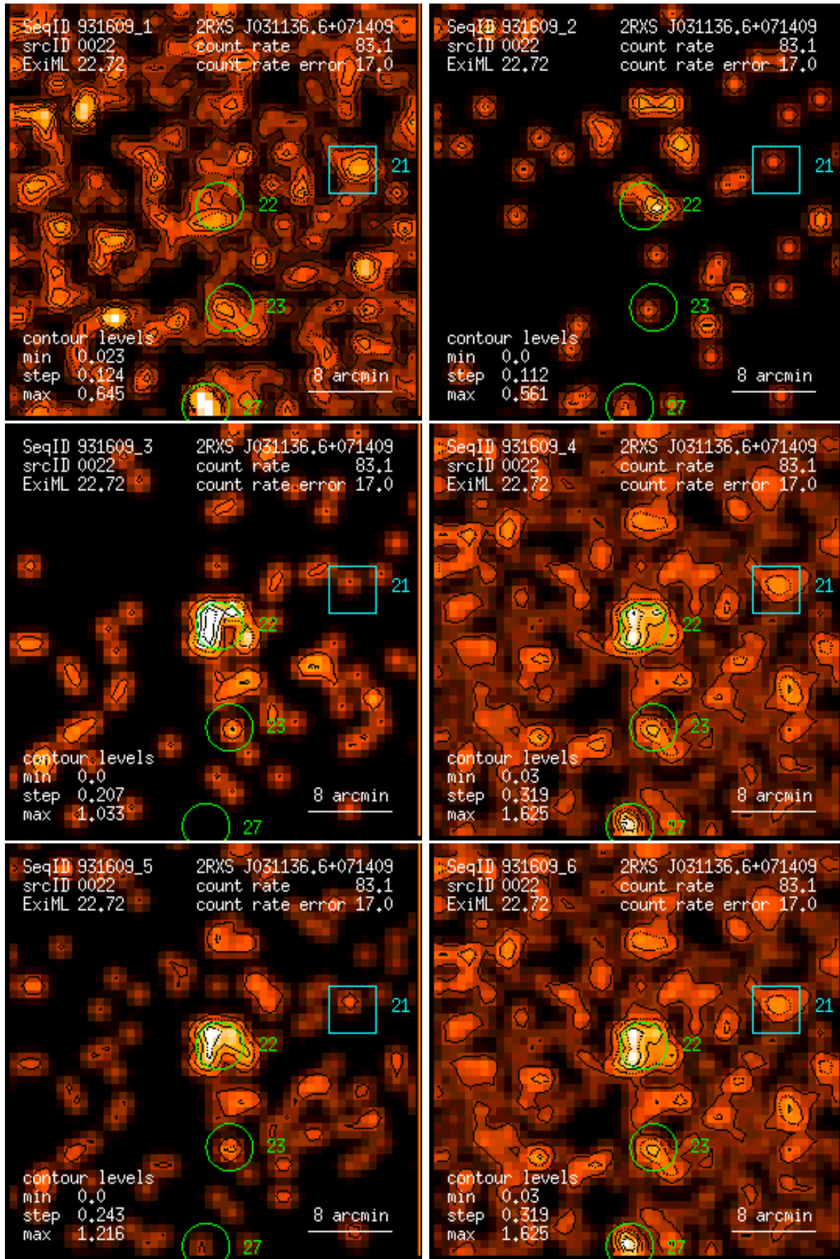
Figure 22: RASS 931609: detection 0022: band rate images, Gaussian filter: (1) PSPC channels 11 – 41, (2) 52 – 90, (3) 91 – 201, (4) 11 – 235, (5) 52 – 201, (6) 11 – 201. Broad band rates in counts/ks. Band rate contour levels in counts/ks/arcmin 2 .
