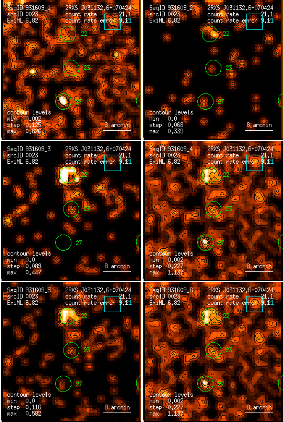
Figure 23: RASS 931609: detection 0023: band rate images, Gaussian filter: (1) PSPC channels 11 – 41, (2) 52 – 90, (3) 91 – 201, (4) 11 – 235, (5) 52 – 201, (6) 11 – 201. Broad band rates in counts/ks. Band rate contour levels in counts/ks/arcmin 2 .
