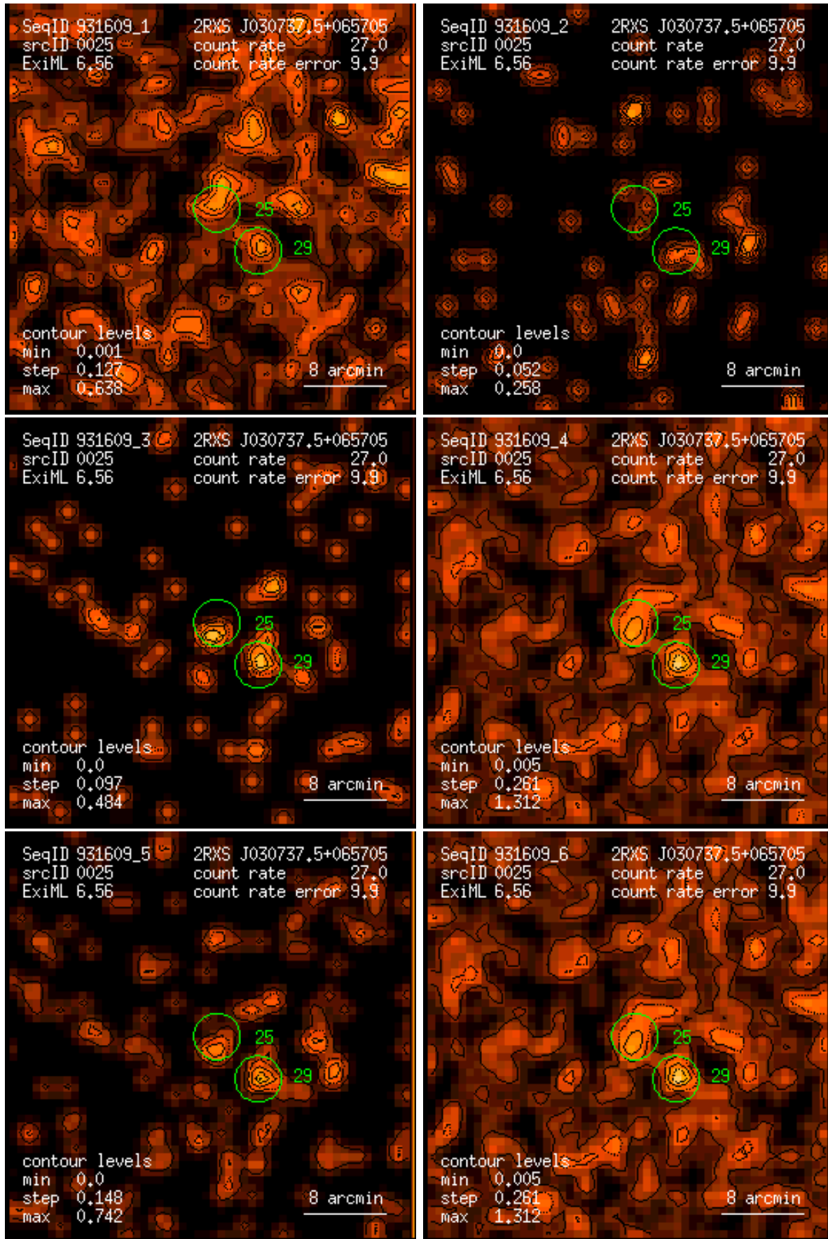
Figure 25: RASS 931609: detection 0025: band rate images, Gaussian filter: (1) PSPC channels 11 – 41, (2) 52 – 90, (3) 91 – 201, (4) 11 – 235, (5) 52 – 201, (6) 11 – 201. Broad band rates in counts/ks. Band rate contour levels in counts/ks/arcmin 2 .
